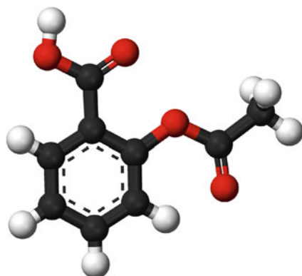
Fig. 6.1: A representation of aspirin, which contains carbon atoms (shown as black balls ) and hydrogen ( white ) and oxygen atoms ( red ). The chemical formula for this molecule is \text{O}=\text{C}(\text{O}c1ccccc1\text{C}(=\text{O})\text{O})\text{O}C , from which molecular descriptors can be determined, such as a molecular weight of 180.2 g/mol
