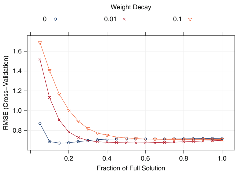
Fig. 6.18: The cross-validation profiles for an elastic net model
