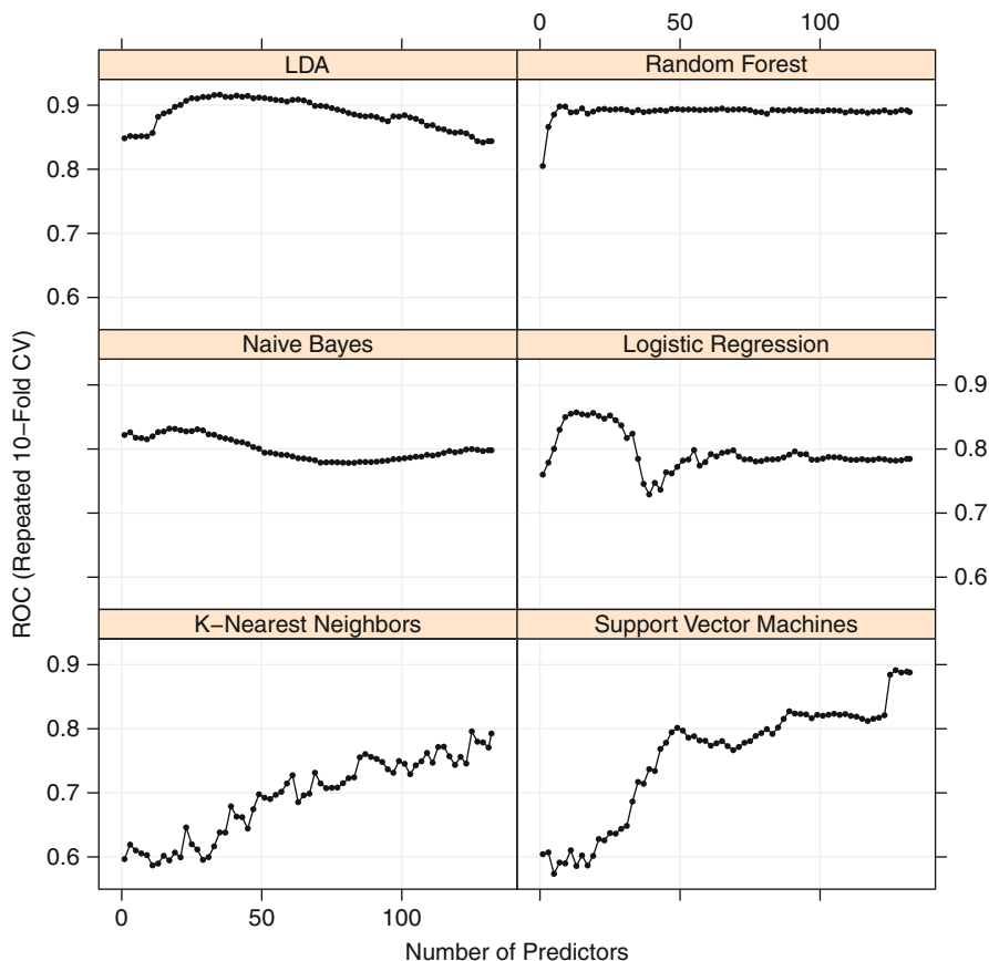
Fig. 19.5: The resampling profiles for the RFE procedure for several models
