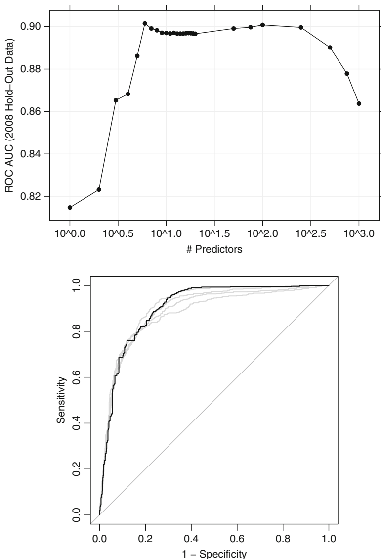
Fig. 12.17: Top : The tuning parameter profile for the sparse LDA model Bottom : The ROC curve for the model (AUC = 0.901)
