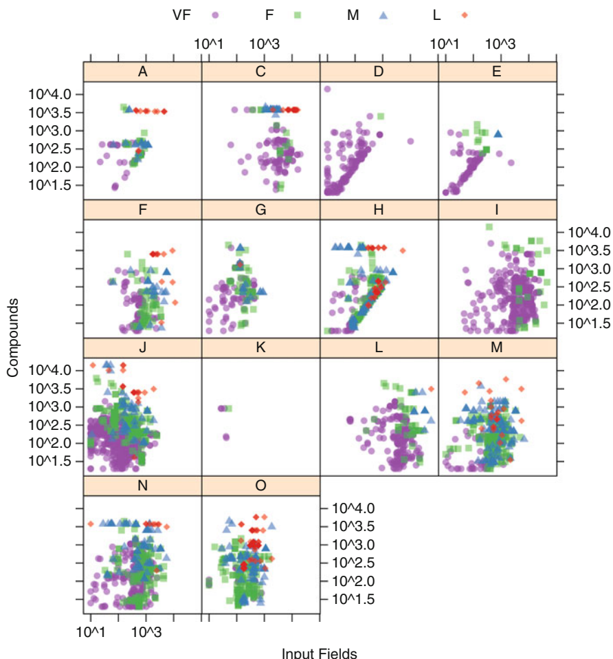
Fig. 17.4: A scatter plot of the number of compounds versus the number of fields for each protocol. The points are colored by their execution time class
