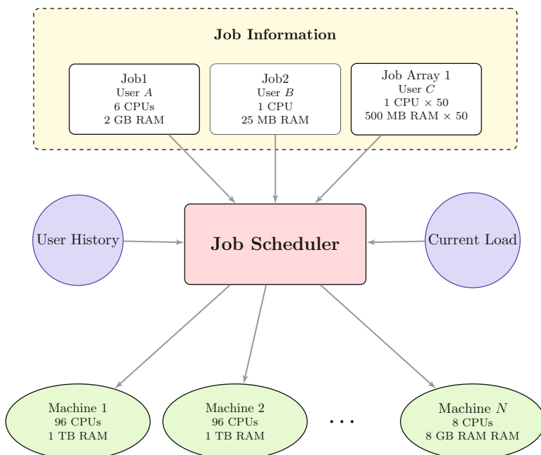
Fig. 17.1: A hypothetical example of a job scheduler in a high-performance computing environment
