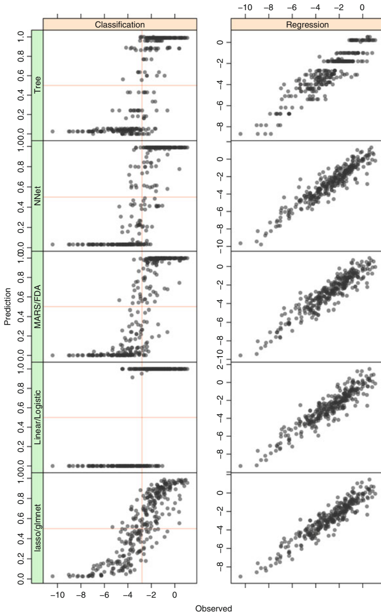
Fig. 20.10: Test set performance comparison of solubility models when the response is modeled as a continuous and categorical value
