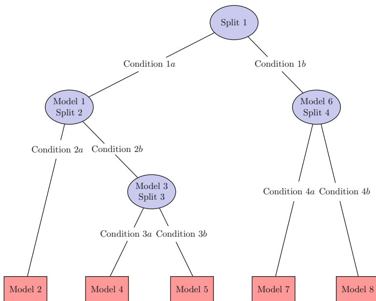
Fig. 8.8: An example of a regression model tree
