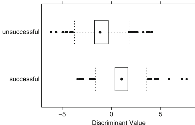
Fig. 12.10: Box plots of the discriminant scores for the 2008 holdout set
