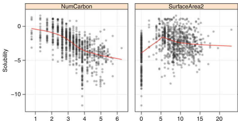
Fig. 18.1: Scatter plots for two numeric predictors (on transformed scales) for the solubility data. The red lines are smoother model fits
