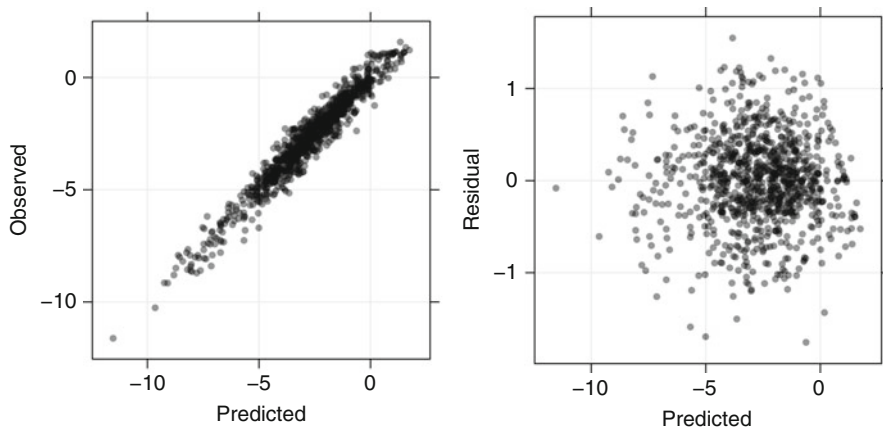
Fig. 6.19: Diagnostic plots for the linear model using the training set. Left : A plot of the observed values versus the predicted values. This plot can show outliers or areas where the model is not calibrated. Right : A plot of the residuals versus predicted values. If the model has been well specified, this plot should be a random cloud of points with no outliers or patterns (e.g., a funnel shape)
