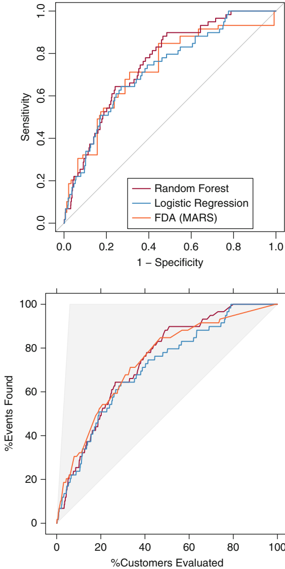
Fig. 16.1: Top : Evaluation set ROC curves for each of the three baseline models. Bottom : The corresponding lift plots
