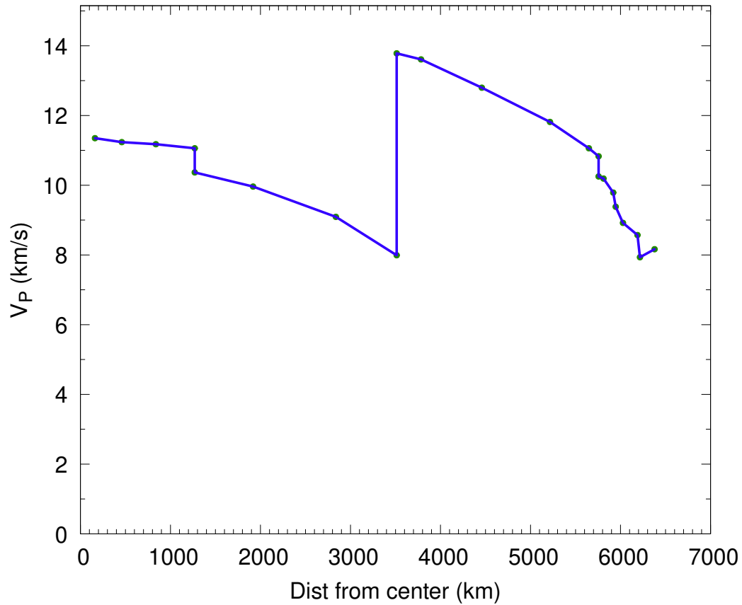
P-wave Velocity
