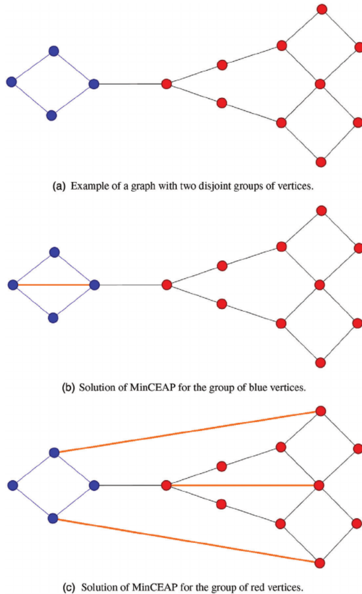
Fig. 3. Example of an instance of problem MinCEAP and its solutions for two groups of vertices. Edges in each solution are represented in orange.
