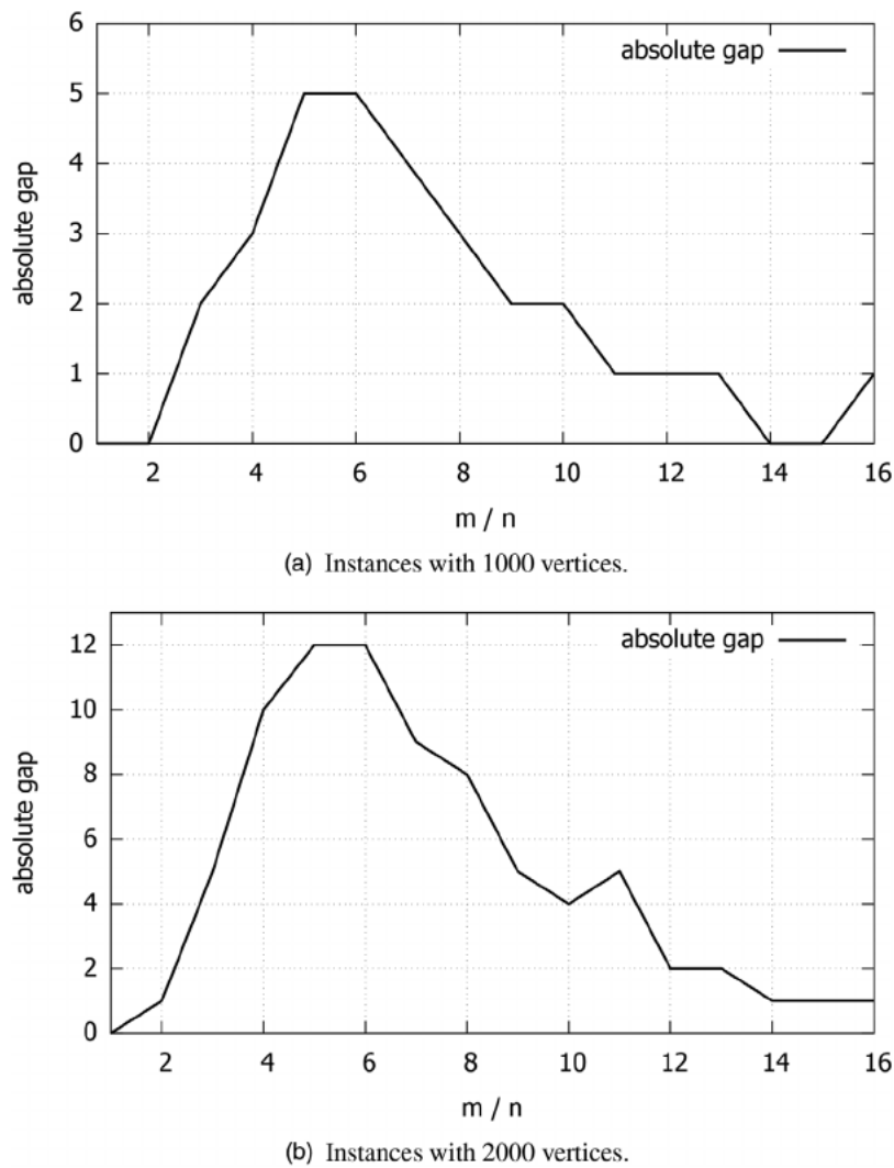
Fig. 6. Variation of the absolute linear relaxation gaps with the increase in the number of edges: on horizontal axis, the ratio m/n between the number of edges and vertices in set A .
