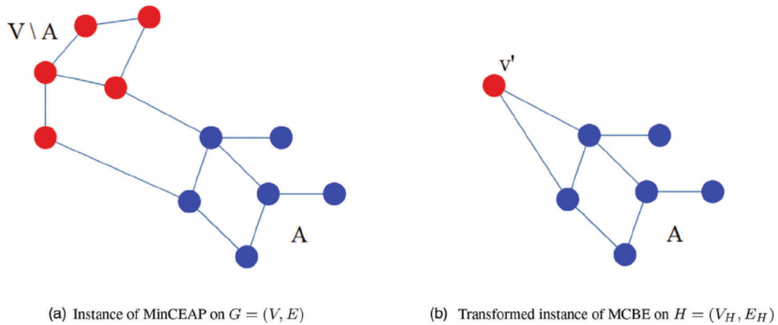
Fig. 5. Instance transformation.
