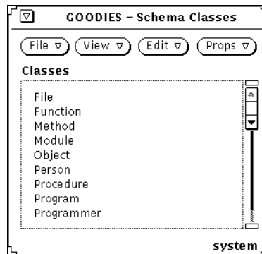
Figure 2: DB Window
