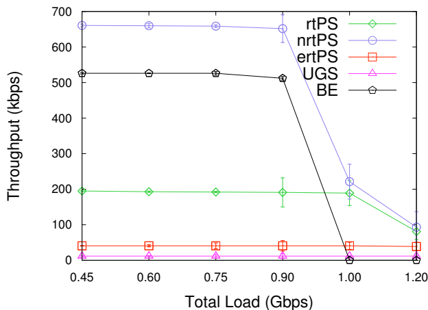
Fig. 2. Throughput of UGS, ertPS, nrtPS, rtPS and BE connections.
