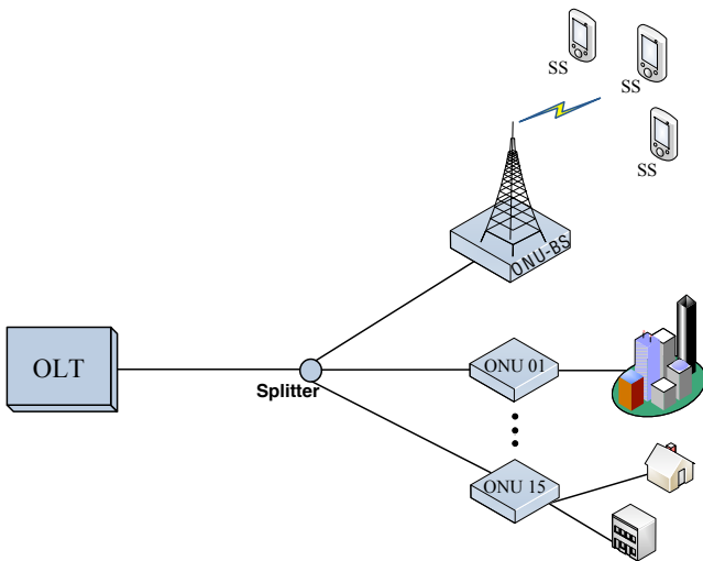
Fig. 1. Integrated architecture of EPON and WiMAX
