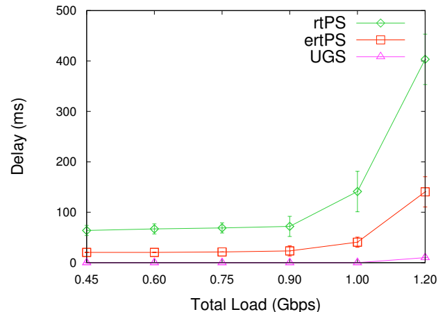
Fig. 3. Latency of UGS, ertPS and rtPS connections.
