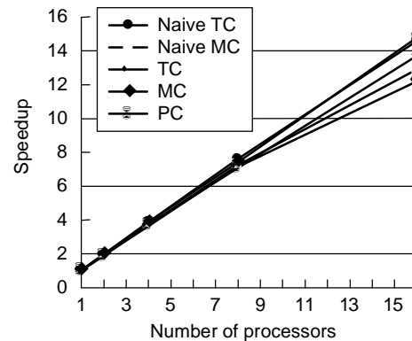
Barnes – Hut
