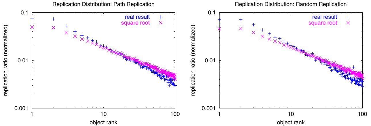
Figure 6: Distribution of replication ratios under Path replication and Random replication.
