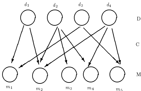
Fig. 1. Causal network of a diagnostic knowledge base KB = \langle D, M, C \rangle .
