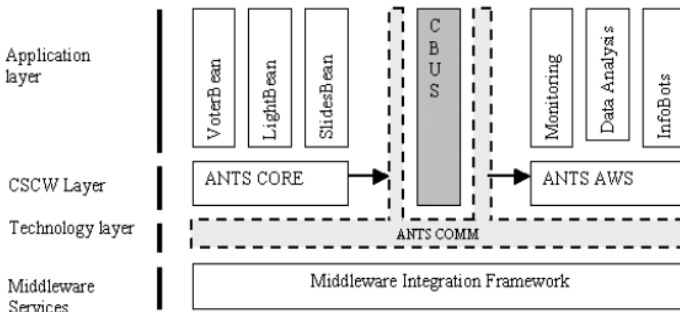
Fig. 5. ANTS framework architecture.
