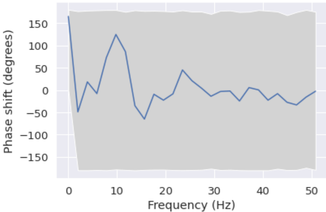
Phase shift for each frequency from Fp2 to O1
