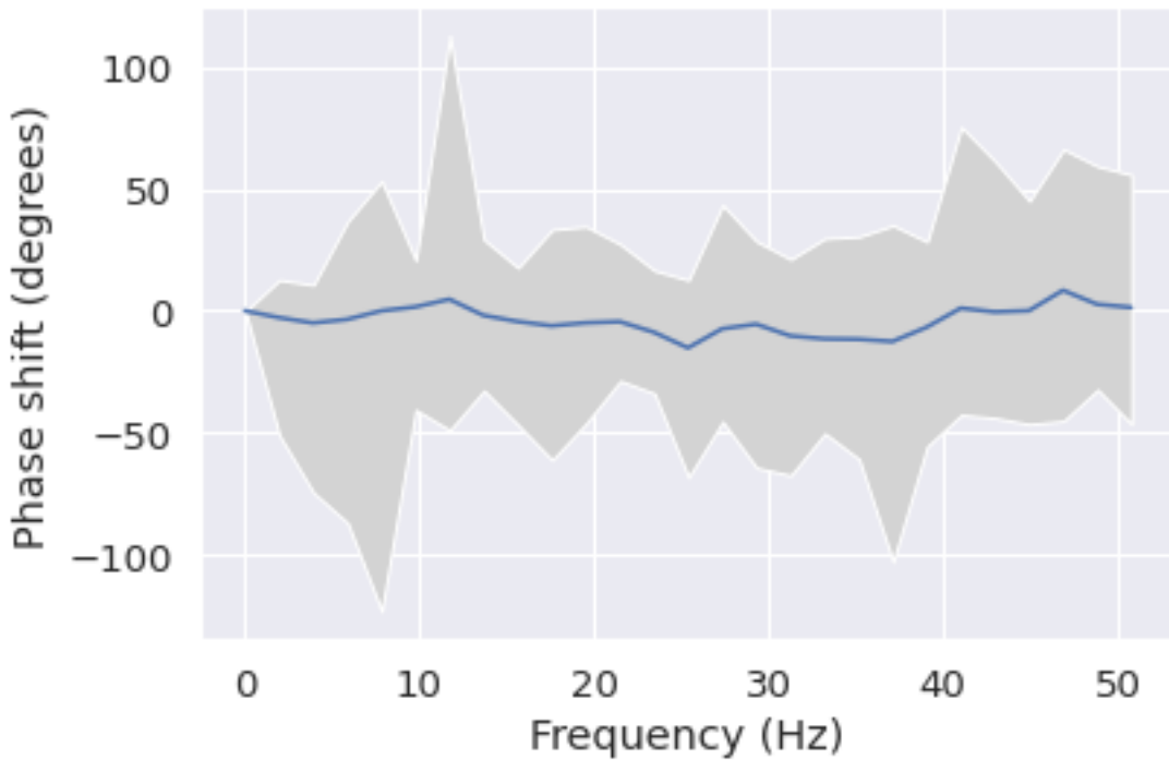
Phase shift for each frequency from Pz to O1
