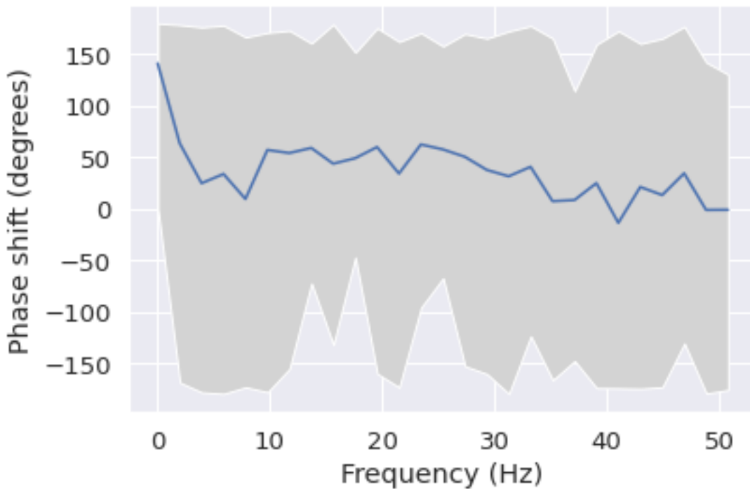
Phase shift for each frequency from Fp1 to T4
