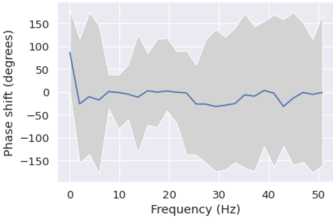
Phase shift for each frequency from F4 to Fp1
