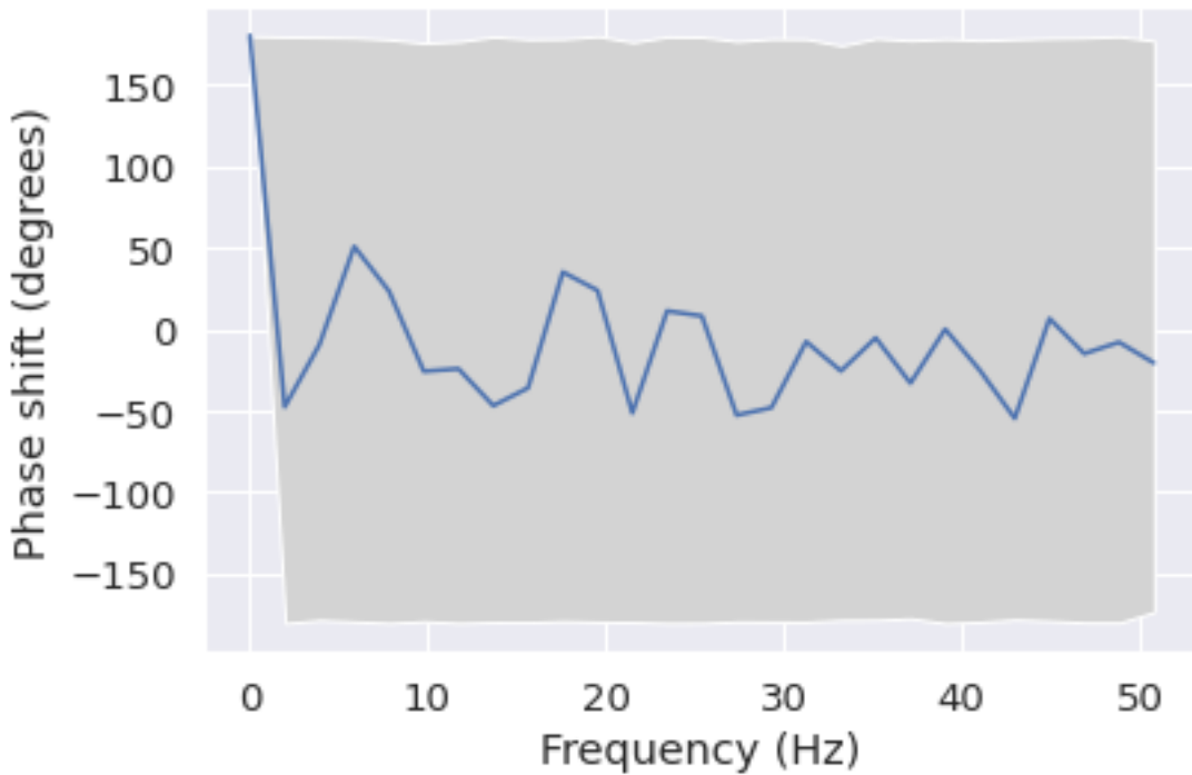
Phase shift for each frequency from Fz to T6
