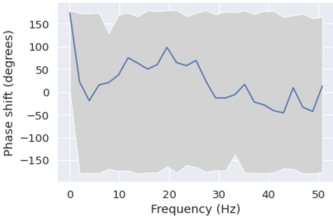
Phase shift for each frequency from Cz to Fp2
