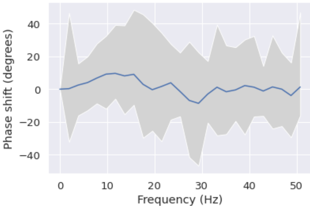
Phase shift for each frequency from T5 to P3
