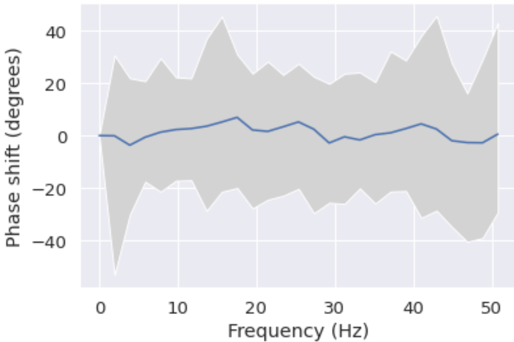
Phase shift for each frequency from F3 to Fp1
