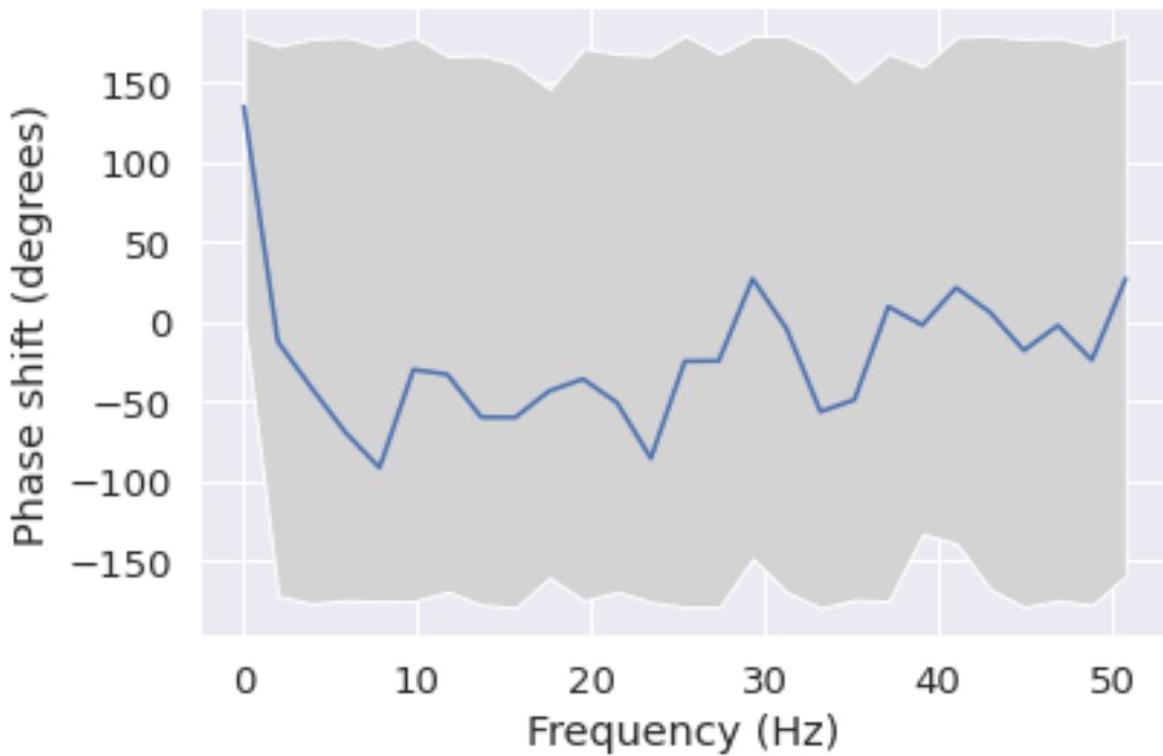
Phase shift for each frequency from T4 to Fp1
