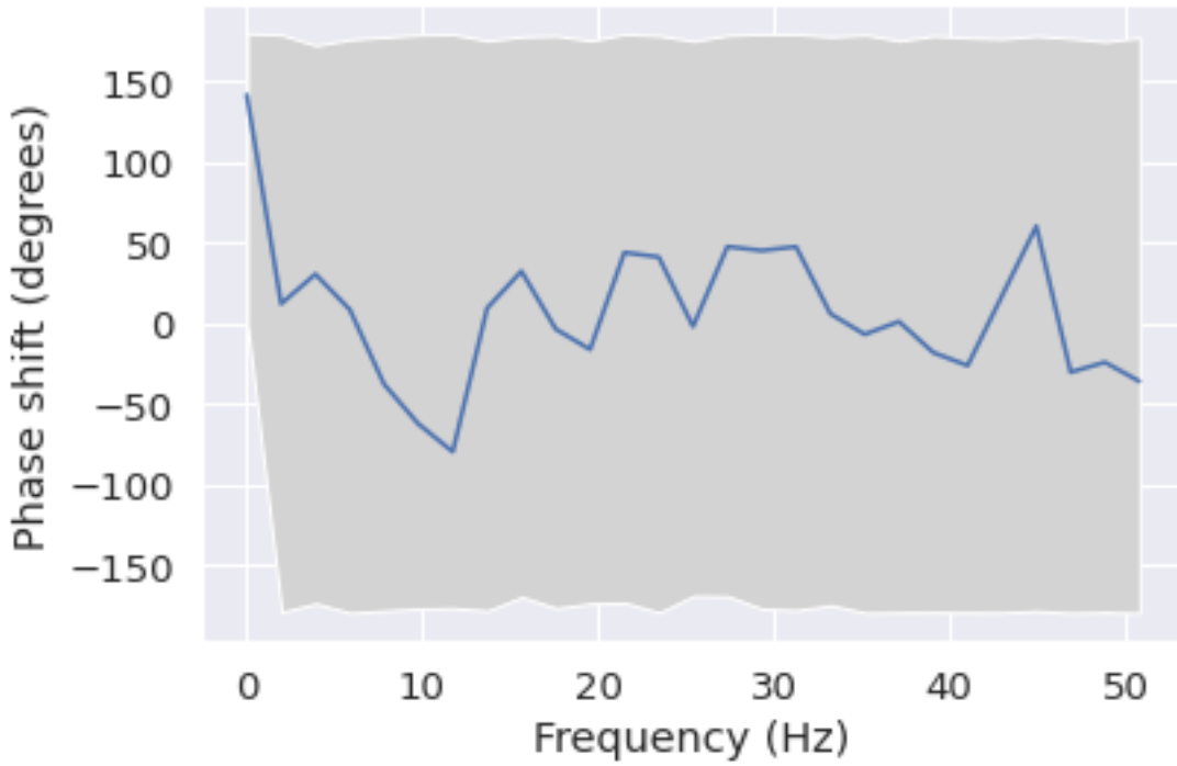
Phase shift for each frequency from C4 to F7
