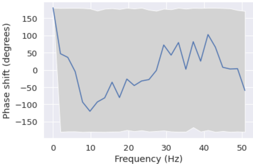
Phase shift for each frequency from O1 to Fp2
