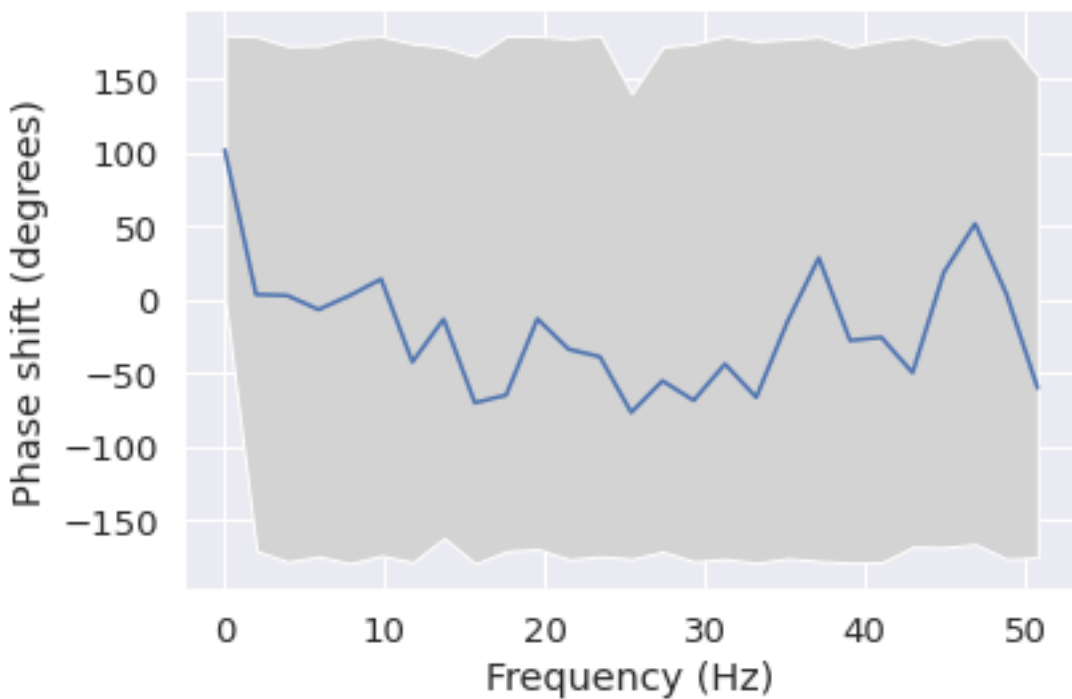
Phase shift for each frequency from F7 to P3
