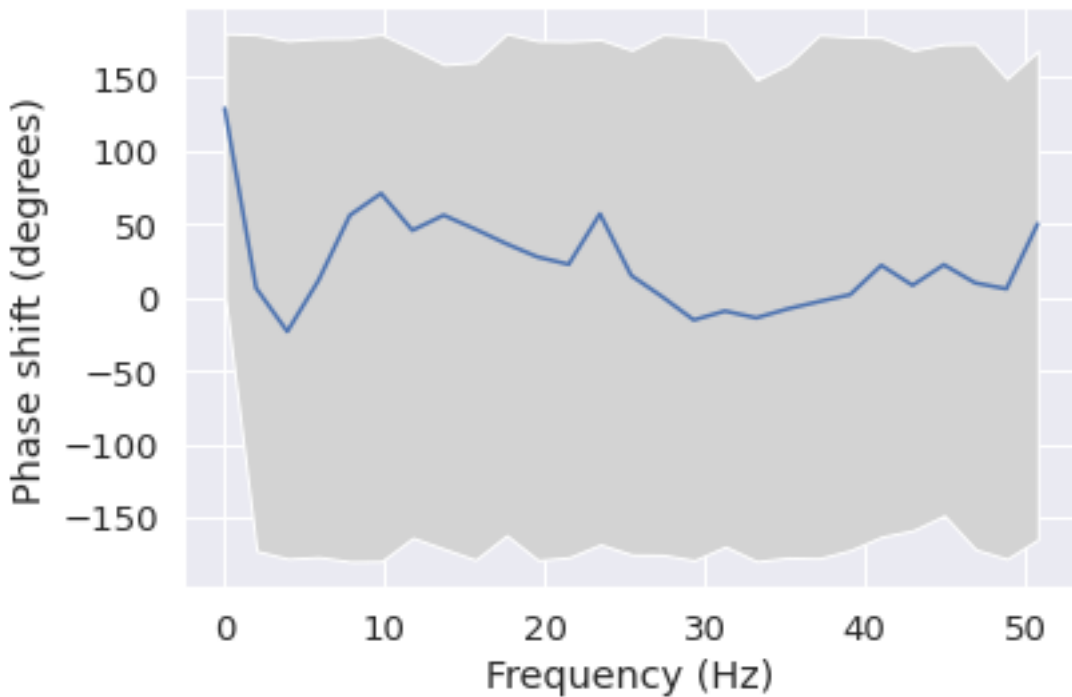
Phase shift for each frequency from Fz to T4
