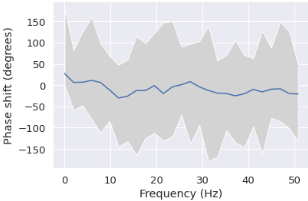
Phase shift for each frequency from Cz to C4
