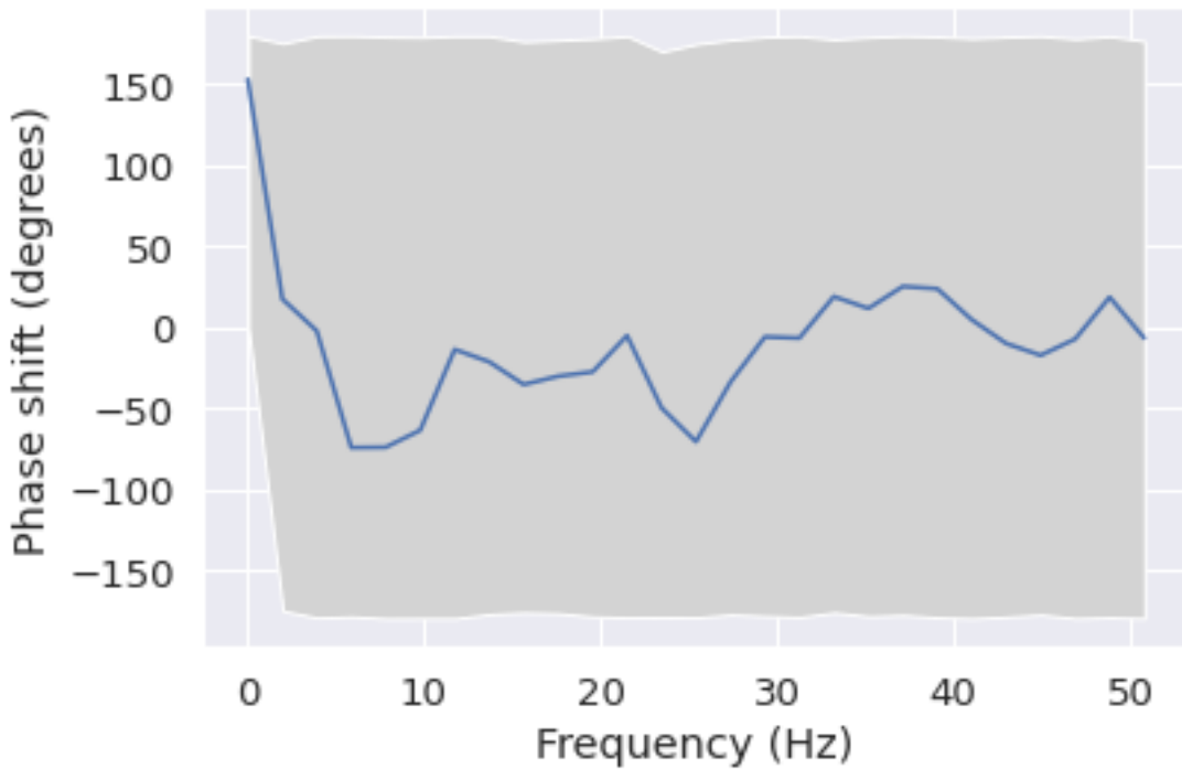
Phase shift for each frequency from C3 to O1
