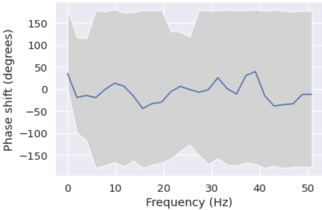
Phase shift for each frequency from P3 to O1
