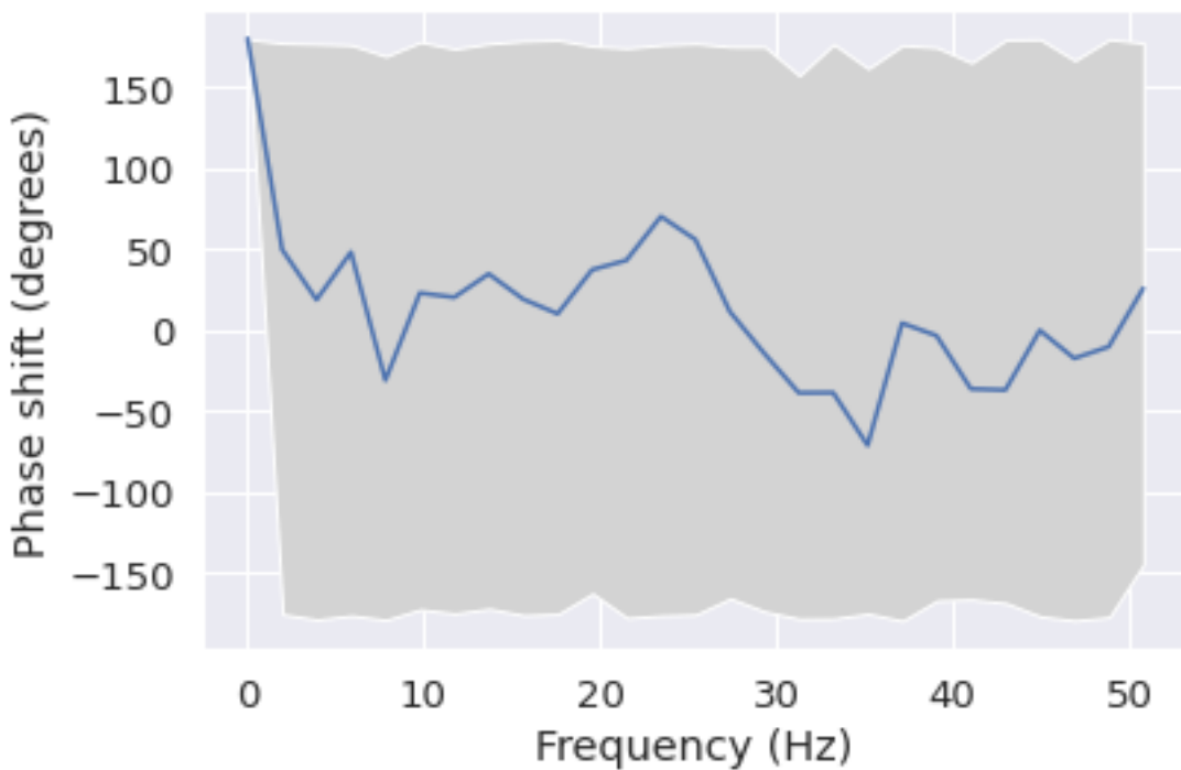
Phase shift for each frequency from Cz to F7
