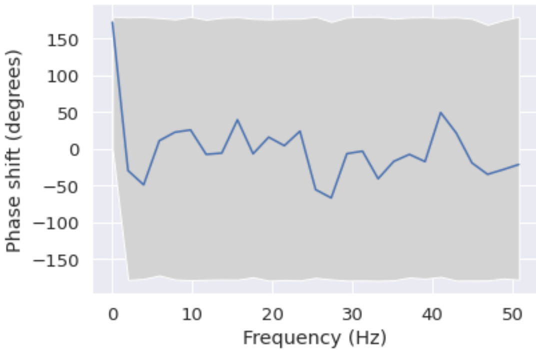
Phase shift for each frequency from F7 to Pz
