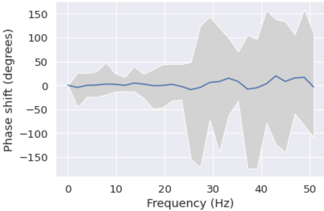
Phase shift for each frequency from Fz to C3
