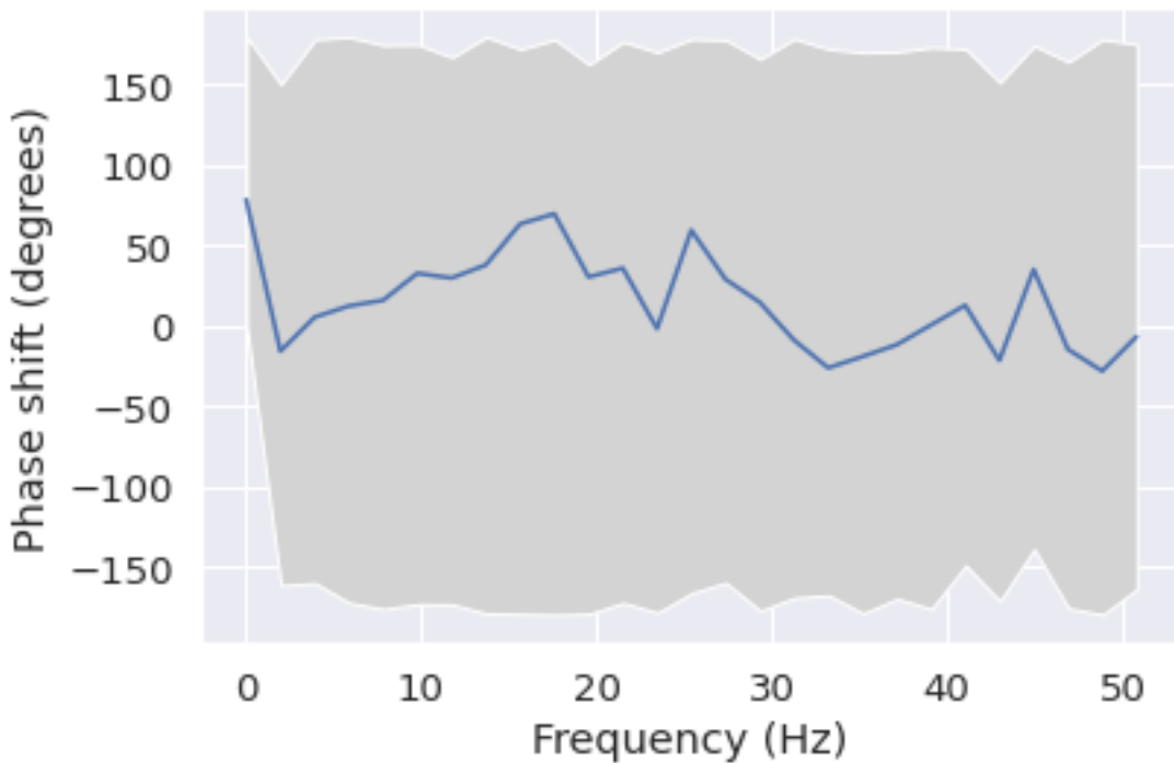
Phase shift for each frequency from P3 to Cz
