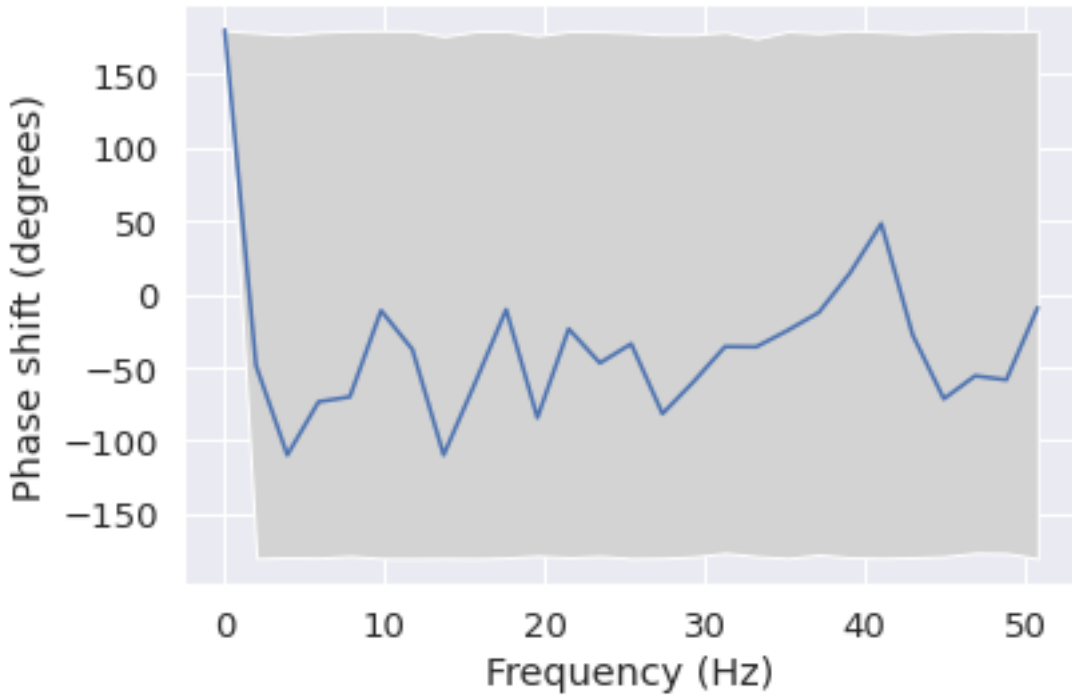
Phase shift for each frequency from Fp2 to Fp1
