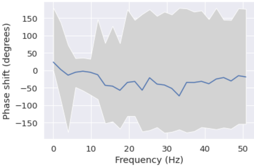
Phase shift for each frequency from P4 to T5
