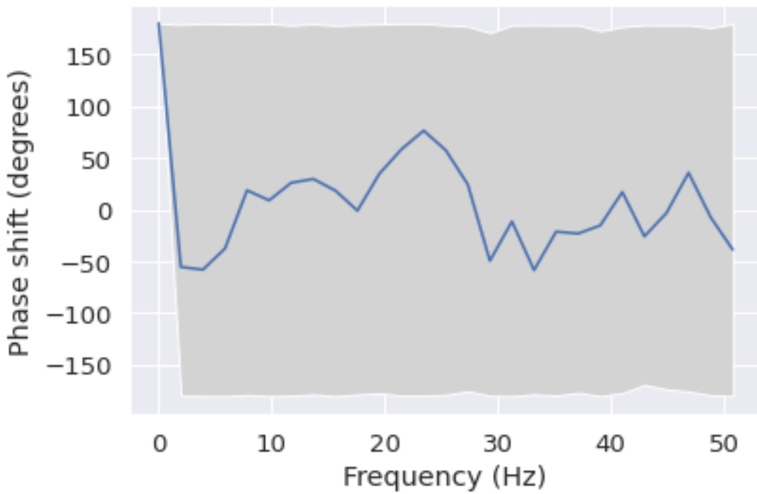
Phase shift for each frequency from F4 to T5
