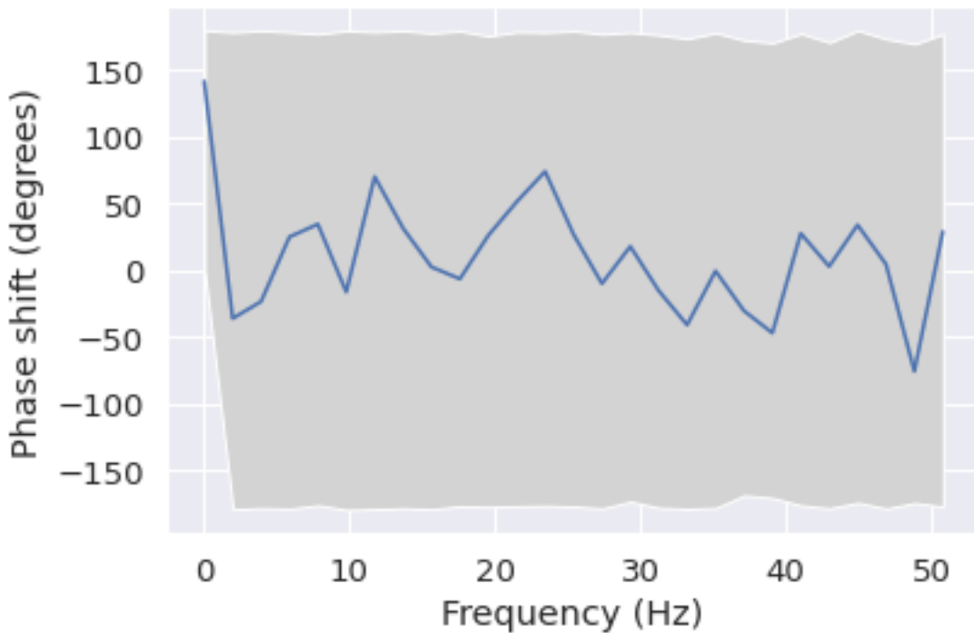
Phase shift for each frequency from O1 to Cz
