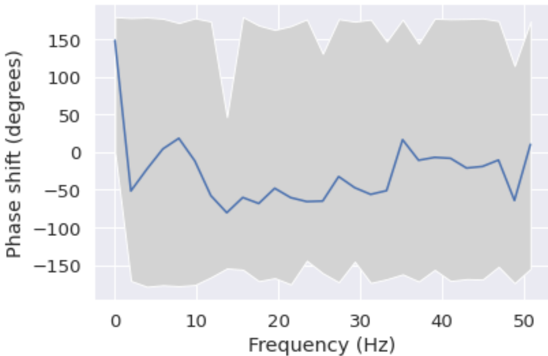
Phase shift for each frequency from T4 to F7
