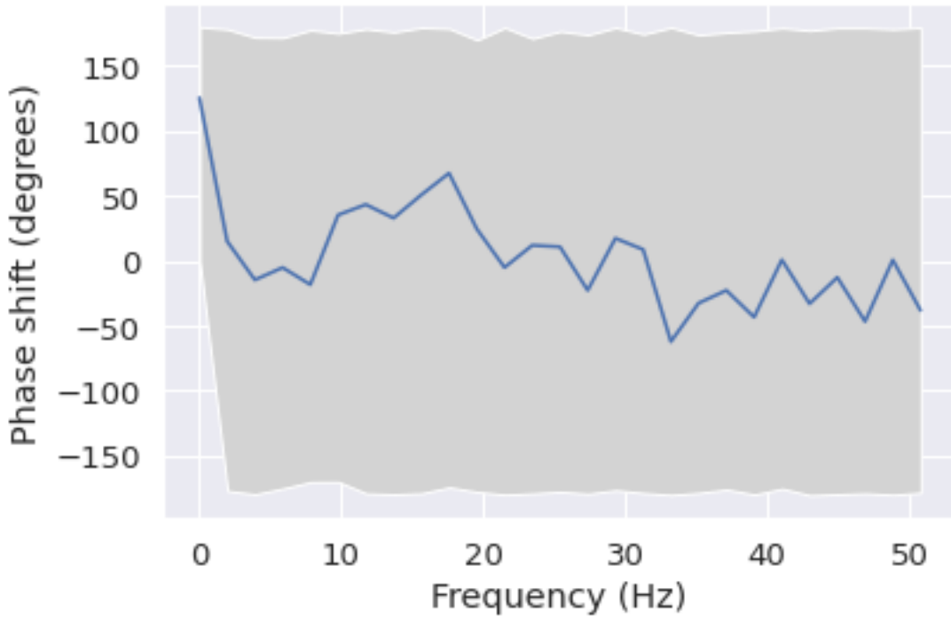
Phase shift for each frequency from T4 to T6
