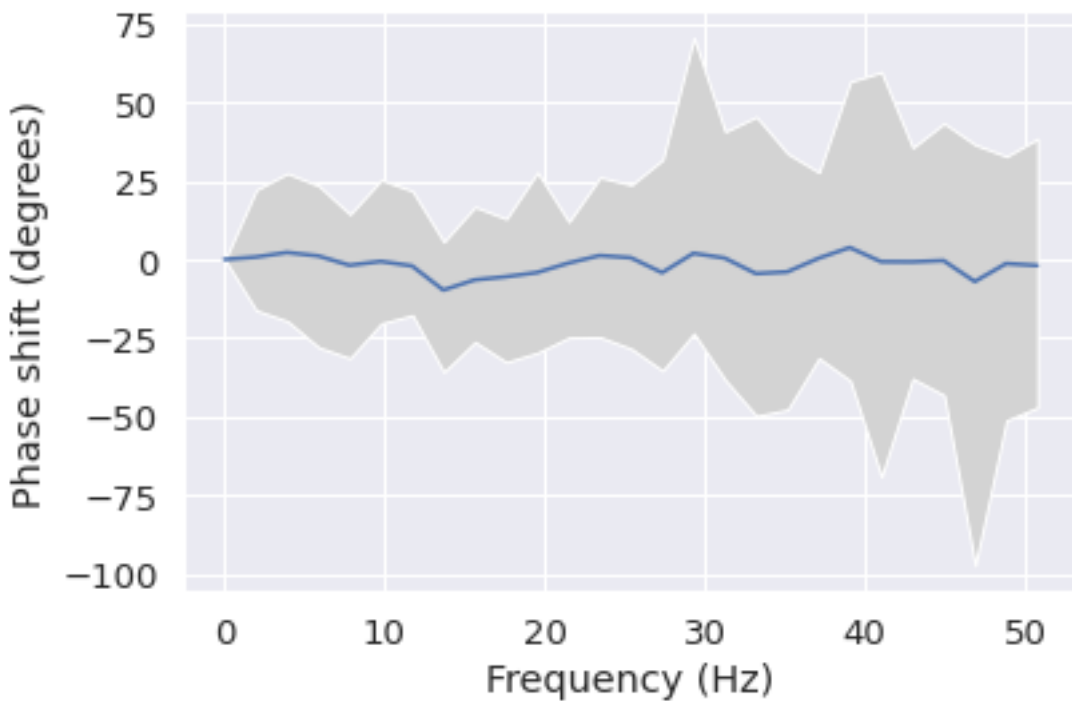
Phase shift for each frequency from F4 to Fz
