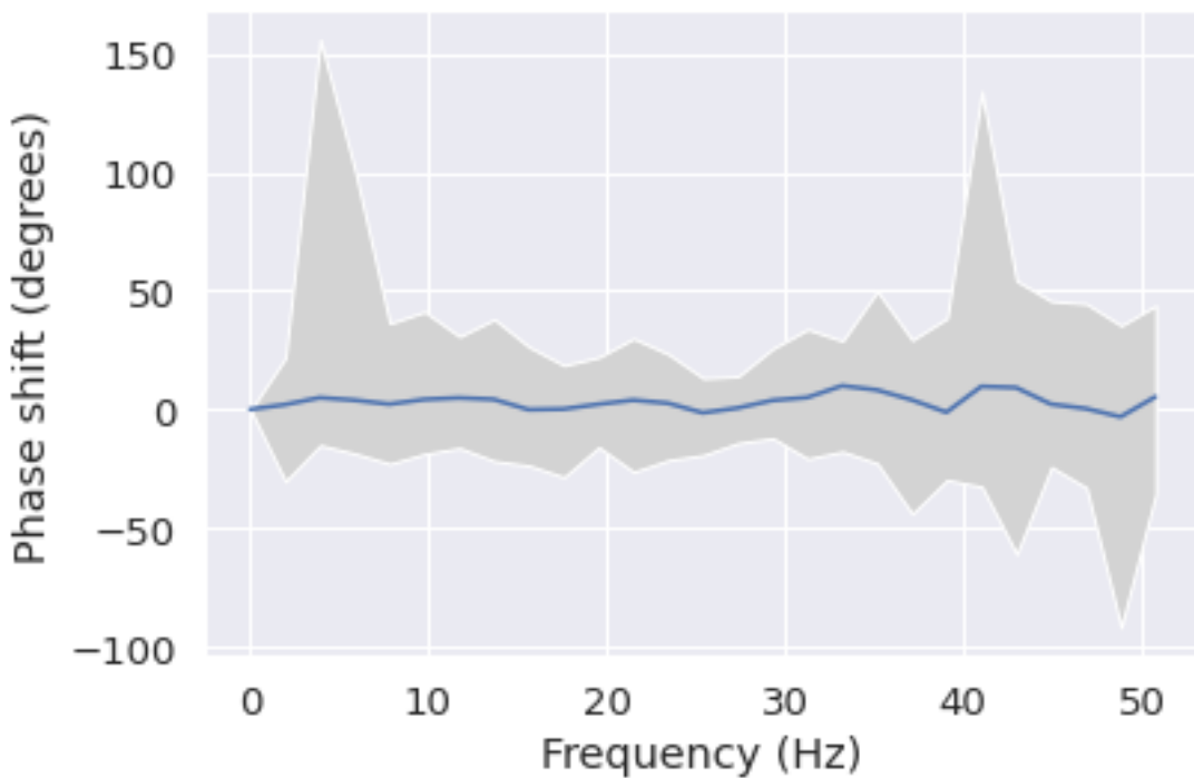
Phase shift for each frequency from Pz to P3
