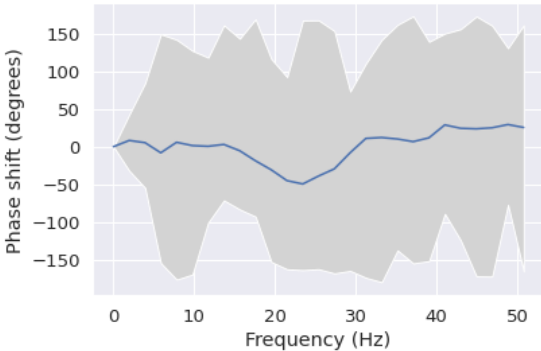
Phase shift for each frequency from Pz to Fp1
