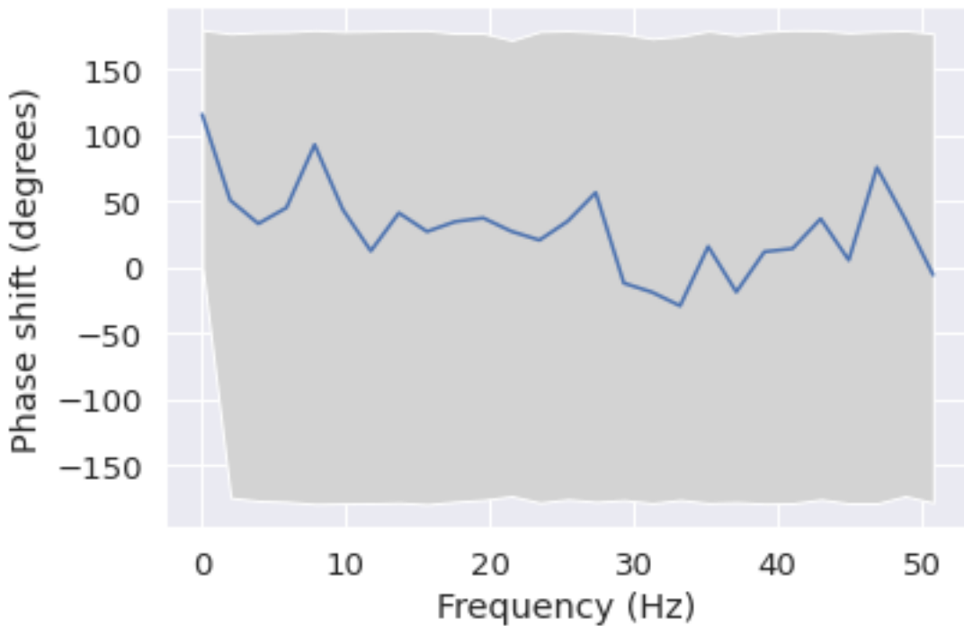
Phase shift for each frequency from P4 to C3
