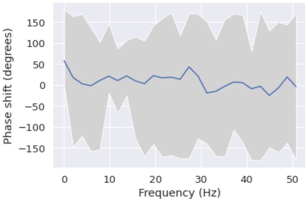
Phase shift for each frequency from F3 to Fp2
