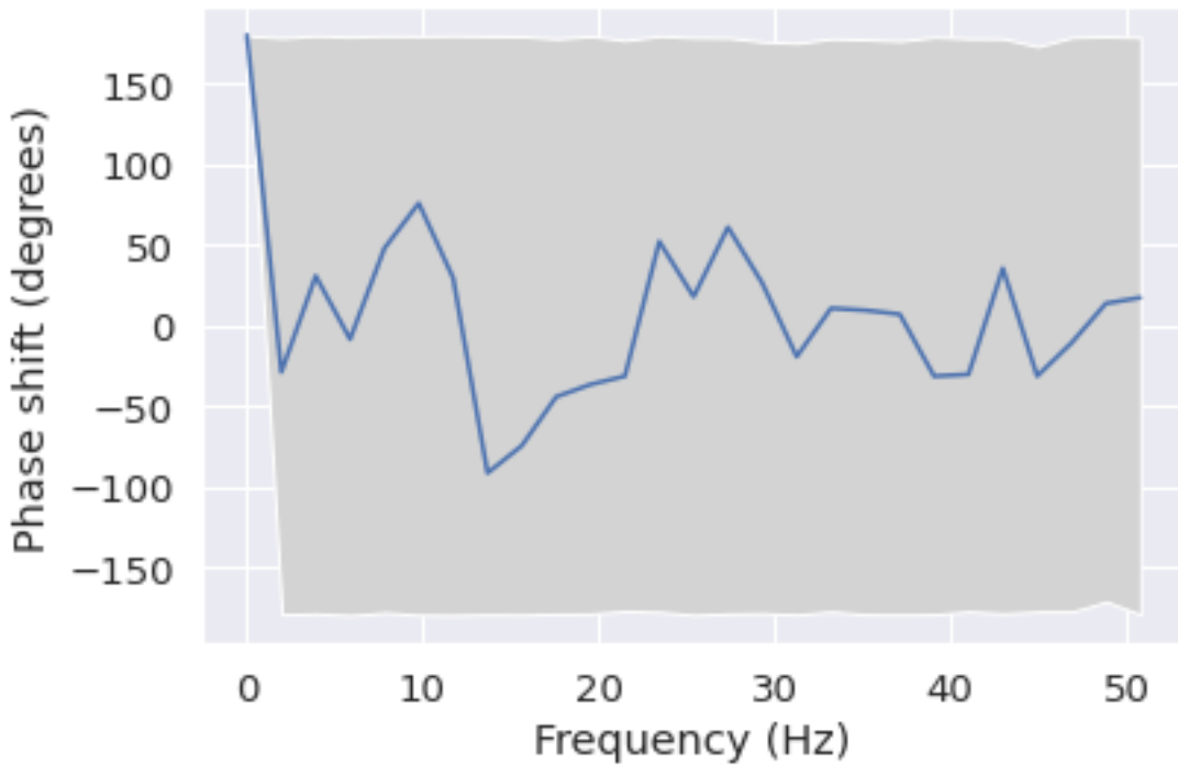
Phase shift for each frequency from Fp2 to P3
