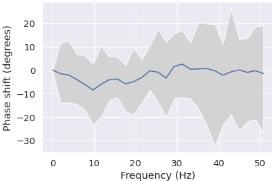
Phase shift for each frequency from T5 to O1
