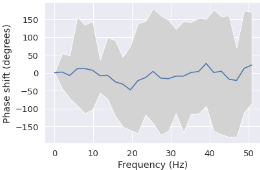
Phase shift for each frequency from T4 to F4
