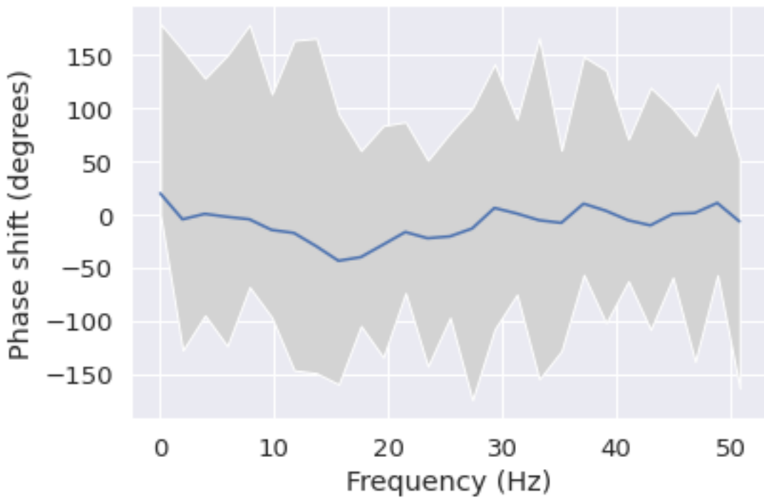
Phase shift for each frequency from Pz to T6
