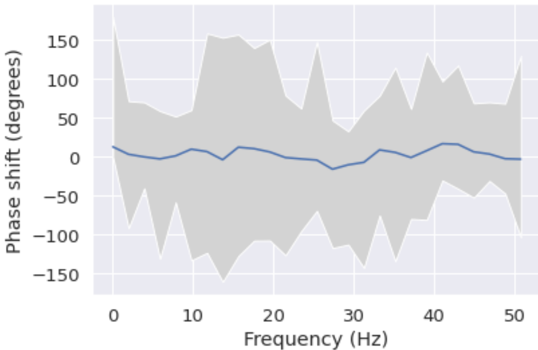
Phase shift for each frequency from C3 to Cz
