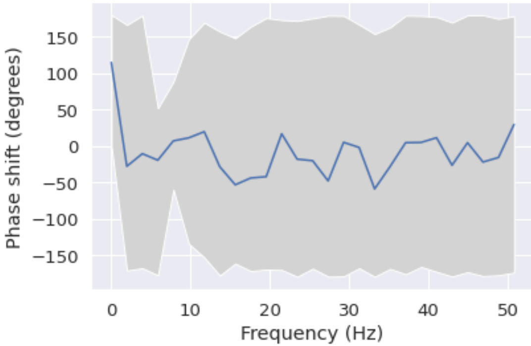
Phase shift for each frequency from C4 to F3
