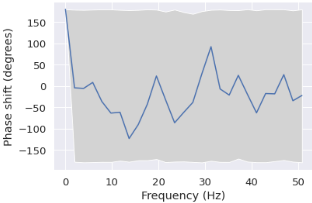
Phase shift for each frequency from T6 to F4
