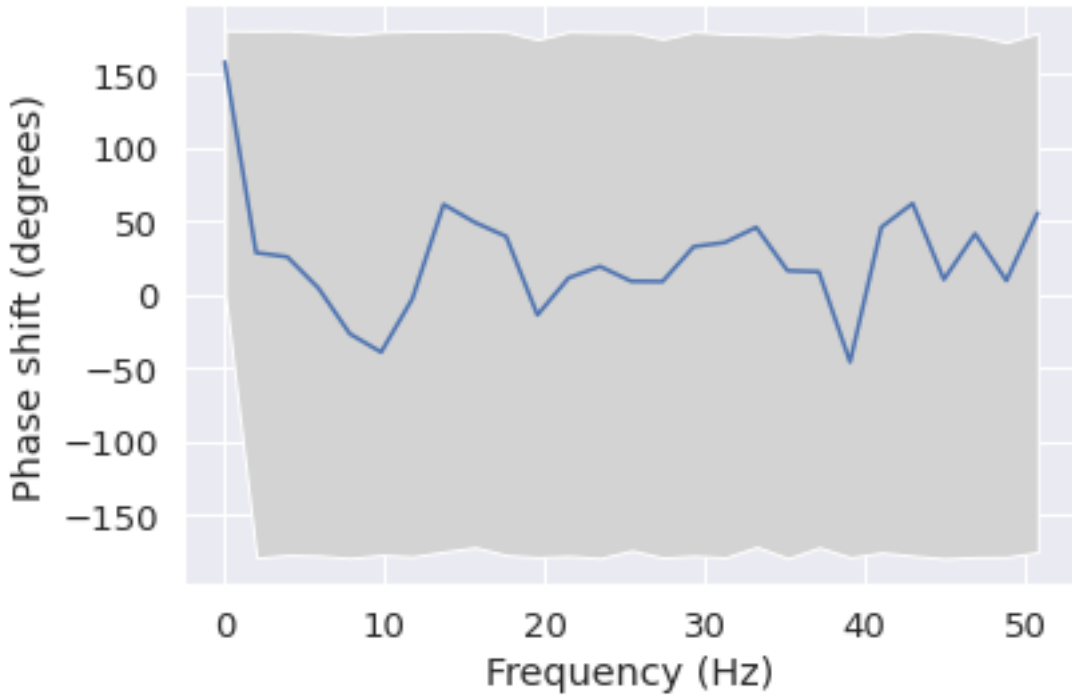
Phase shift for each frequency from Fp1 to P3
