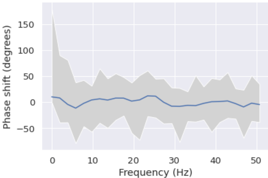
Phase shift for each frequency from Fz to Fp1
