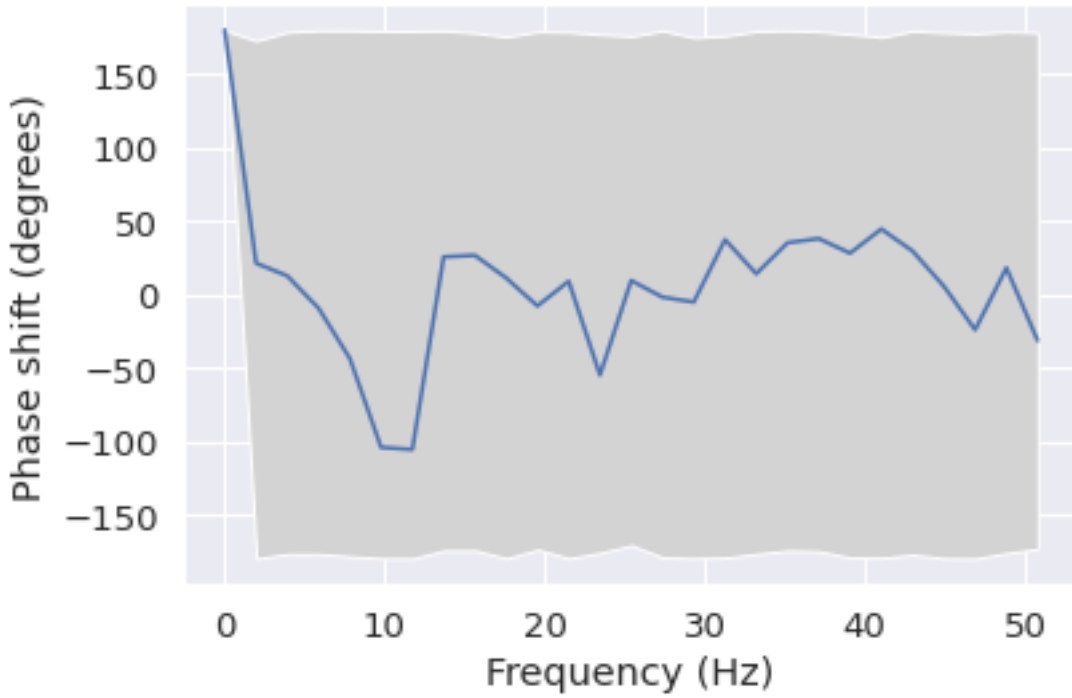
Phase shift for each frequency from T5 to F3
