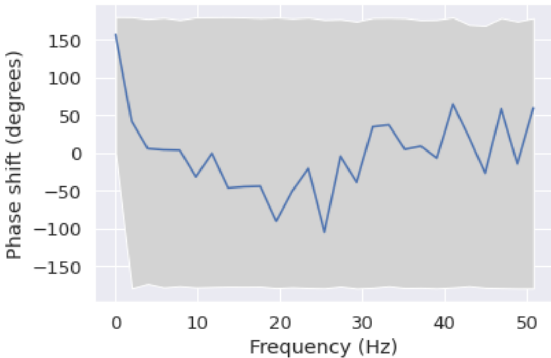
Phase shift for each frequency from Fz to Pz
