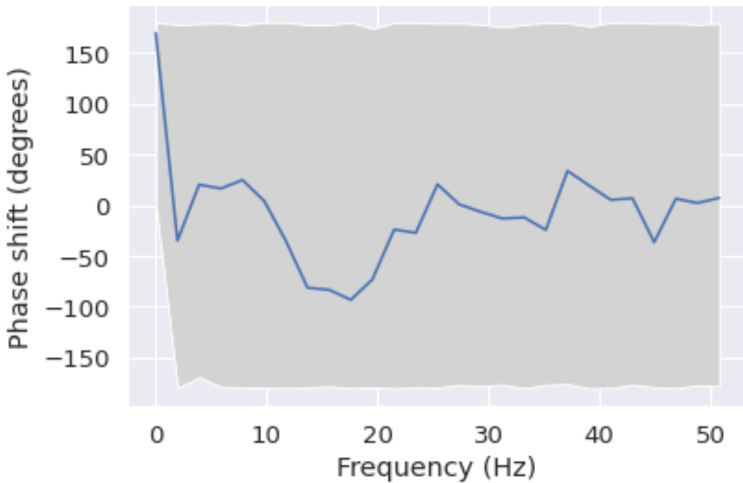
Phase shift for each frequency from T5 to P3
