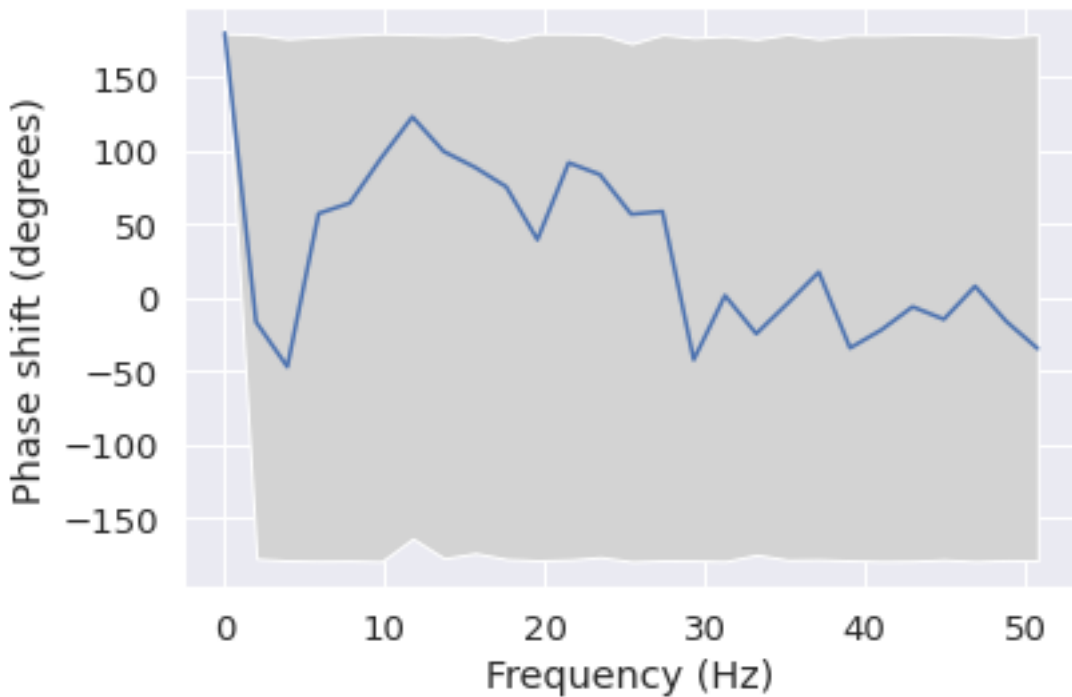
Phase shift for each frequency from Fp1 to T6
