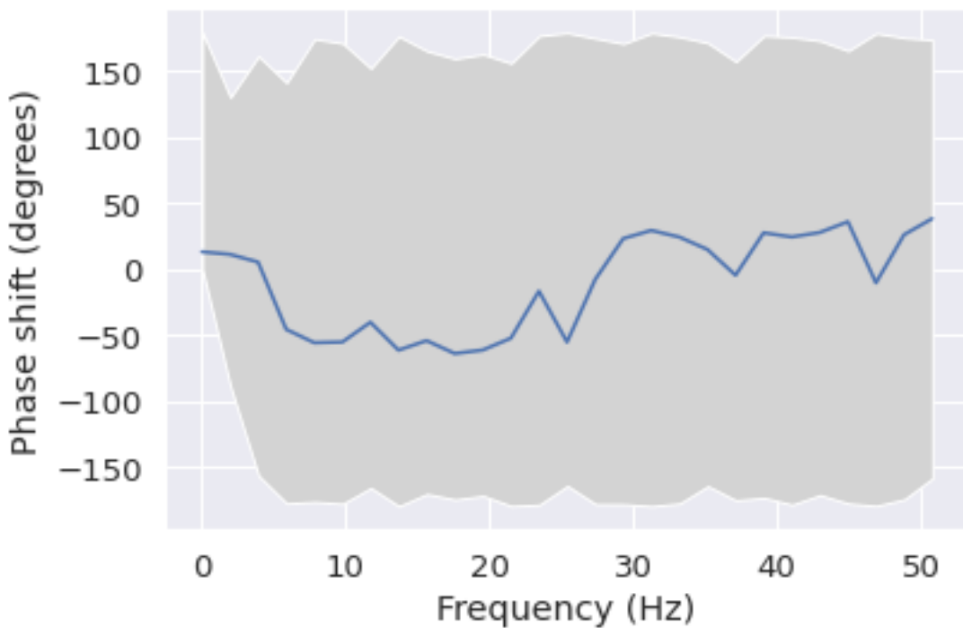
Phase shift for each frequency from Cz to P4
