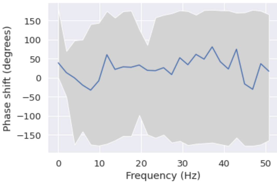
Phase shift for each frequency from P4 to P3
