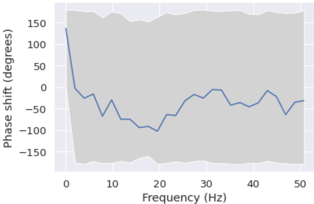
Phase shift for each frequency from F7 to O1
