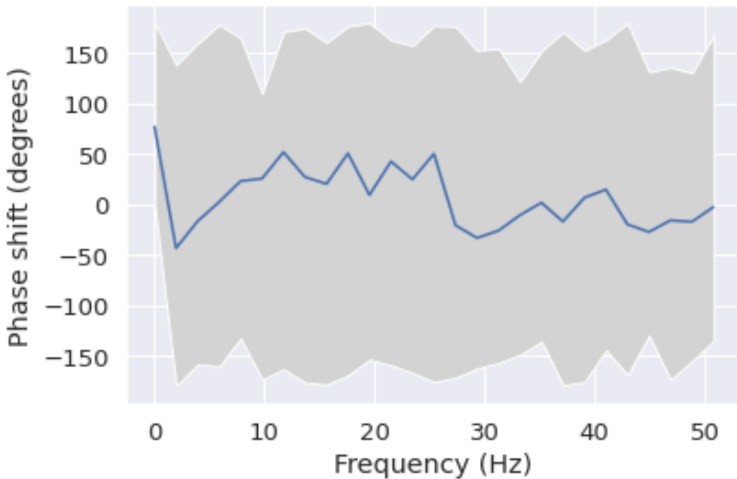
Phase shift for each frequency from C4 to Fz
