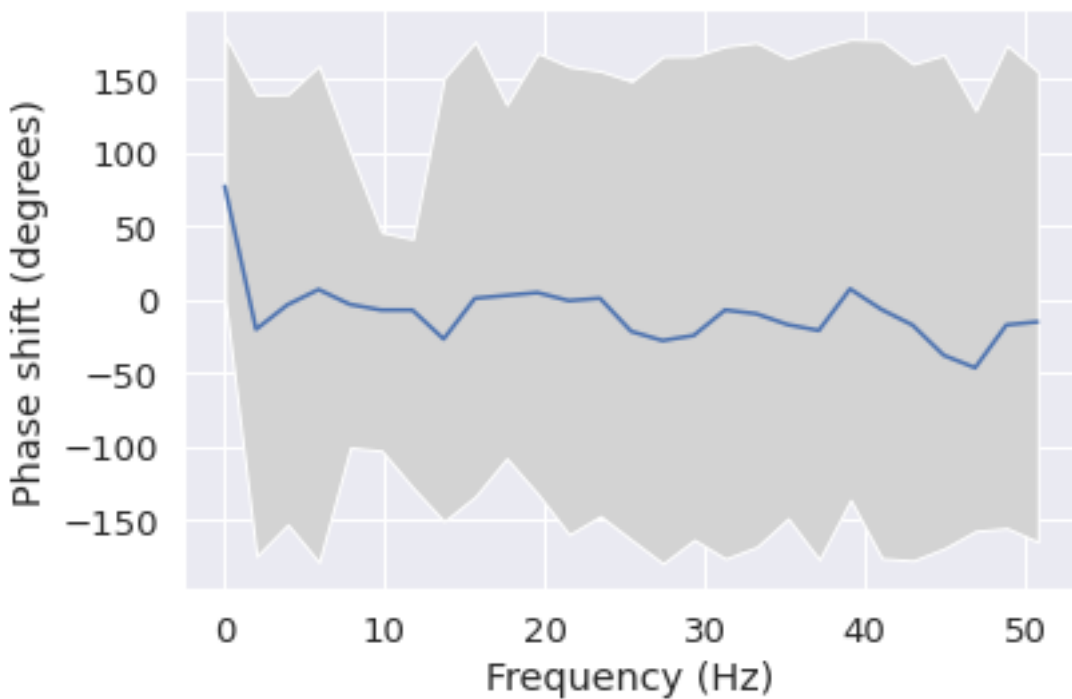
Phase shift for each frequency from F4 to F3
