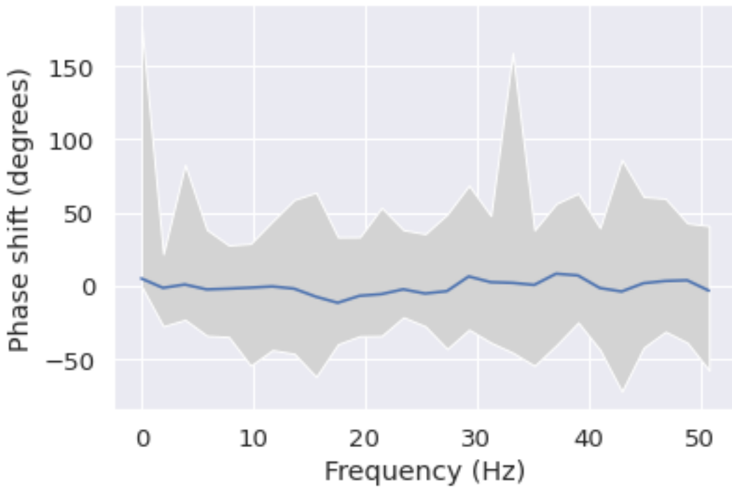
Phase shift for each frequency from Pz to O1
