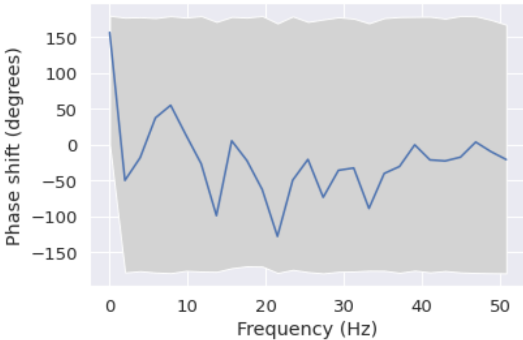
Phase shift for each frequency from P4 to Fp2
