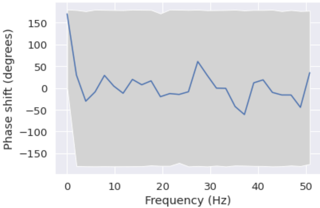
Phase shift for each frequency from Pz to T4
