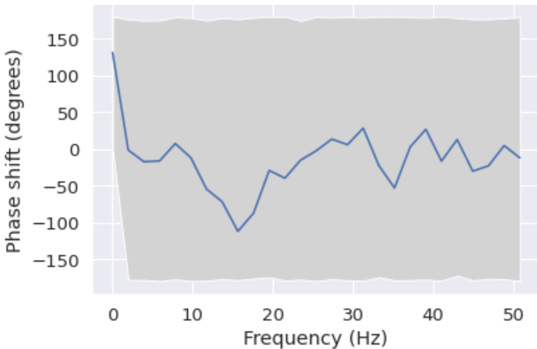
Phase shift for each frequency from O1 to C4
