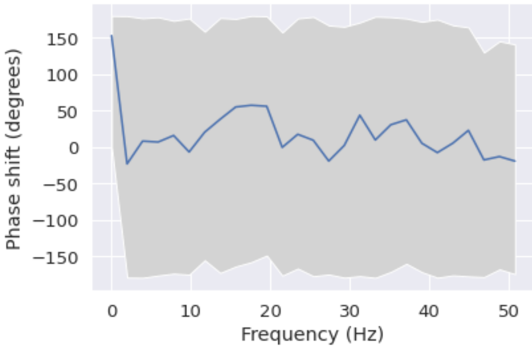
Phase shift for each frequency from F7 to C3
