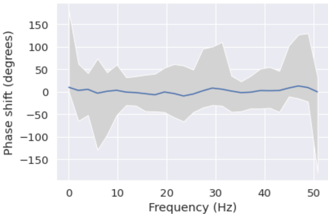
Phase shift for each frequency from F7 to F3
