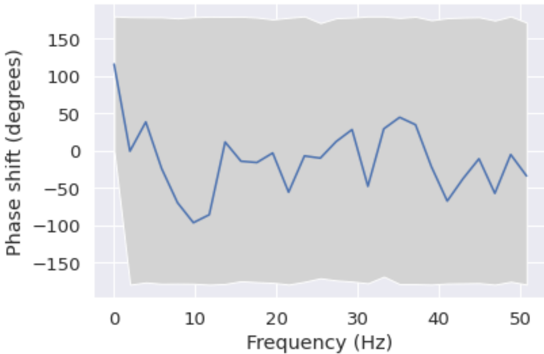
Phase shift for each frequency from C4 to P4
