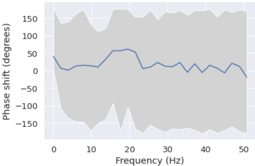
Phase shift for each frequency from T5 to T4
