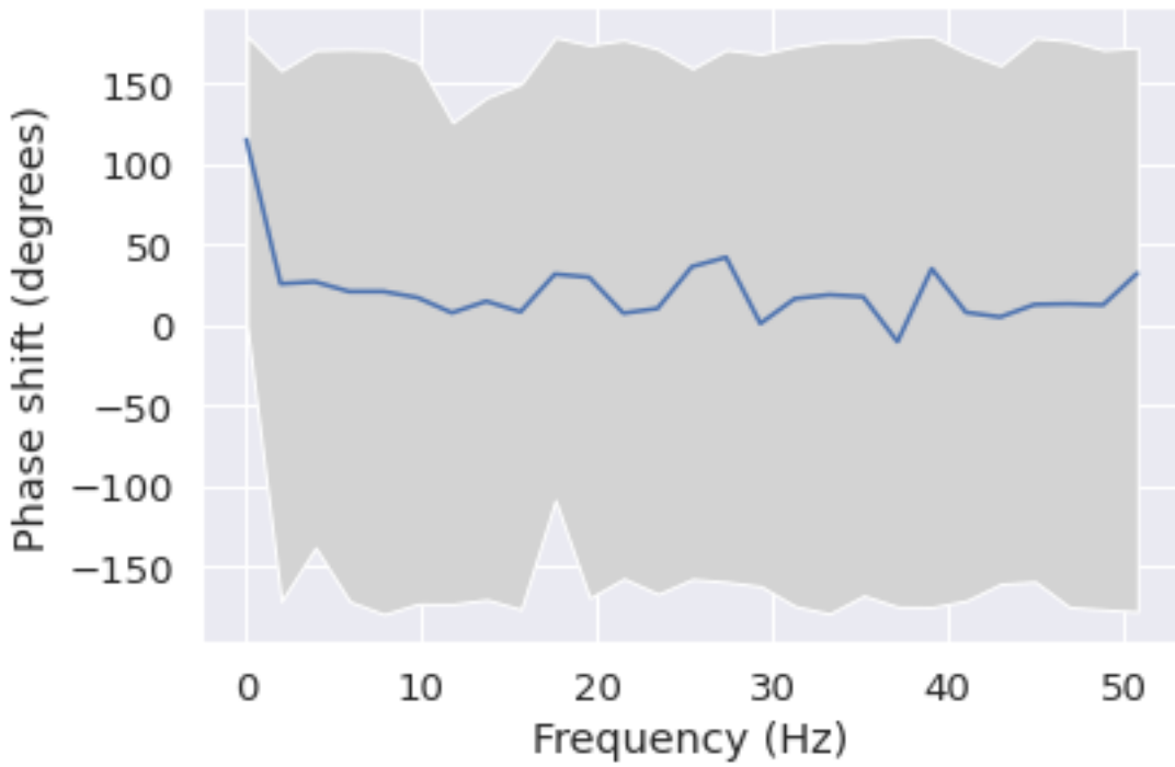
Phase shift for each frequency from F3 to C3
