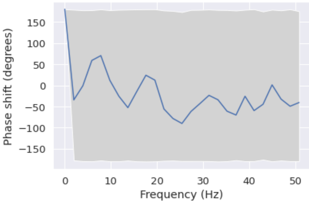
Phase shift for each frequency from Pz to Fp2
