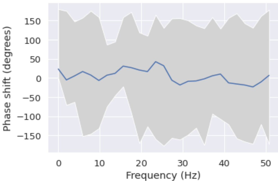
Phase shift for each frequency from Pz to Cz
