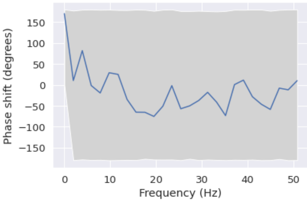
Phase shift for each frequency from C3 to T6
