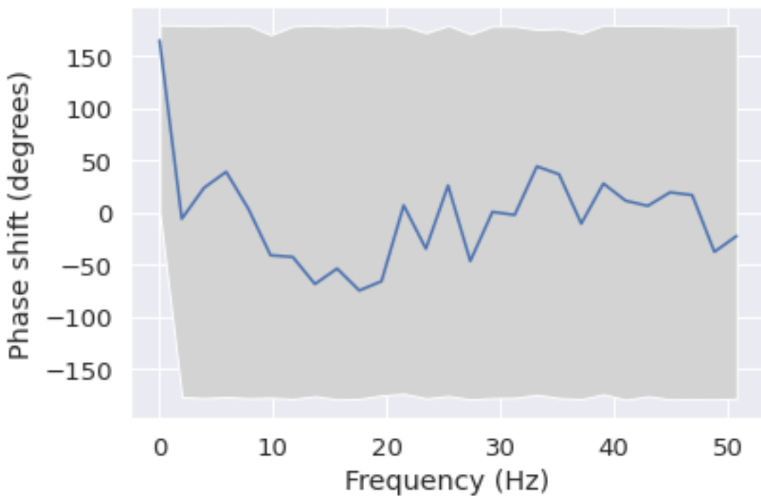
Phase shift for each frequency from P3 to T4
