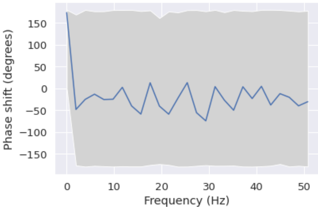
Phase shift for each frequency from F3 to O1
