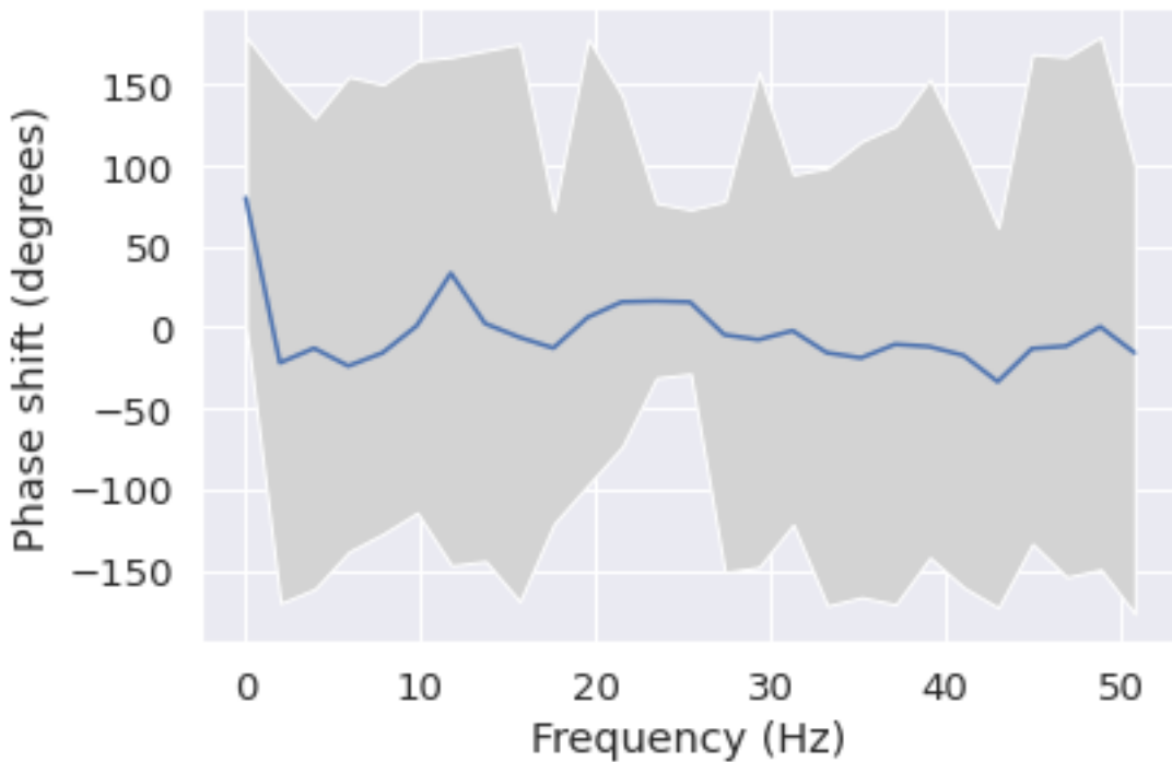
Phase shift for each frequency from T5 to Pz
