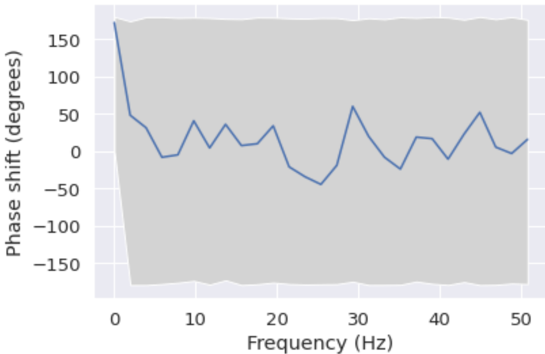
Phase shift for each frequency from C4 to T5
