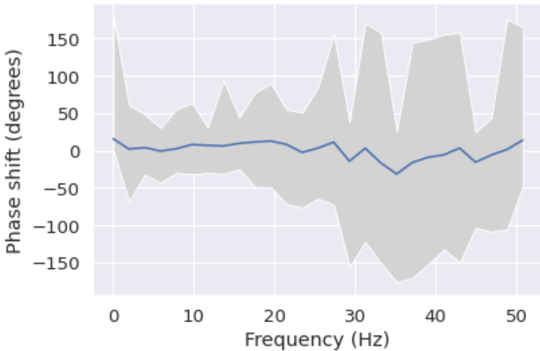
Phase shift for each frequency from F3 to T4
