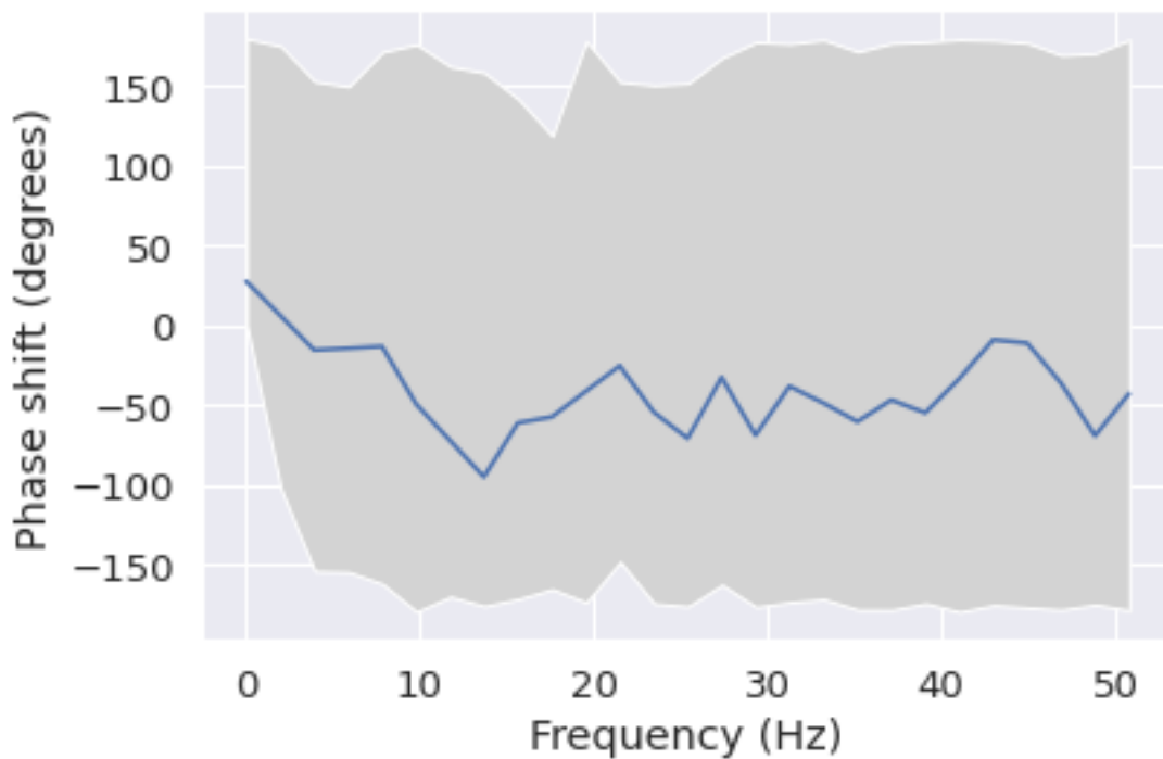
Phase shift for each frequency from P3 to T6
