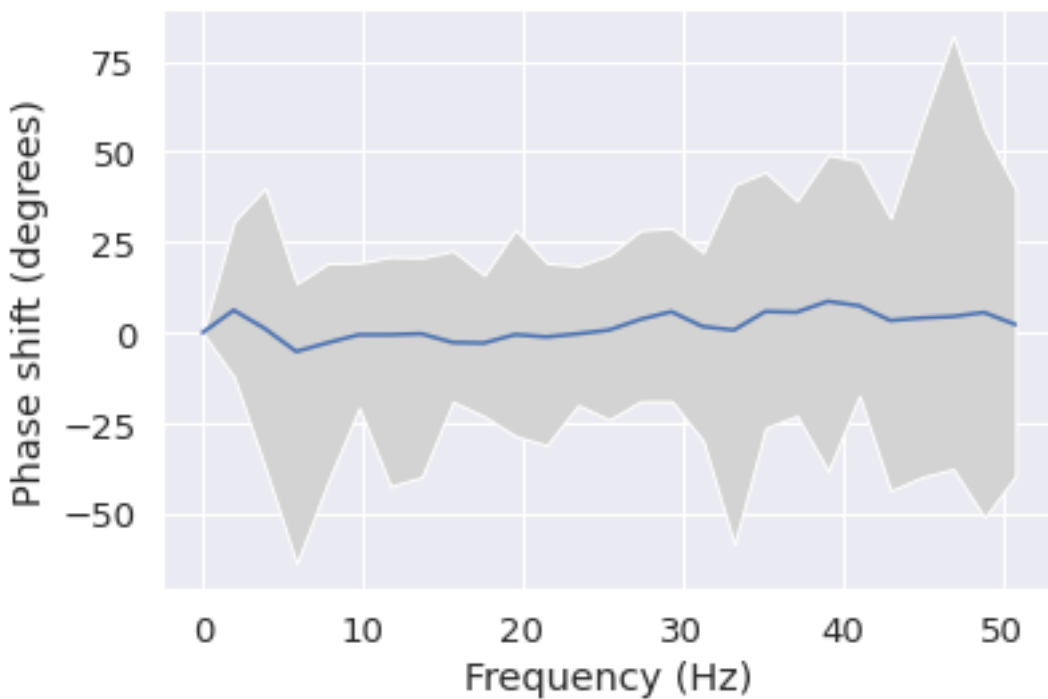
Phase shift for each frequency from Pz to P3
