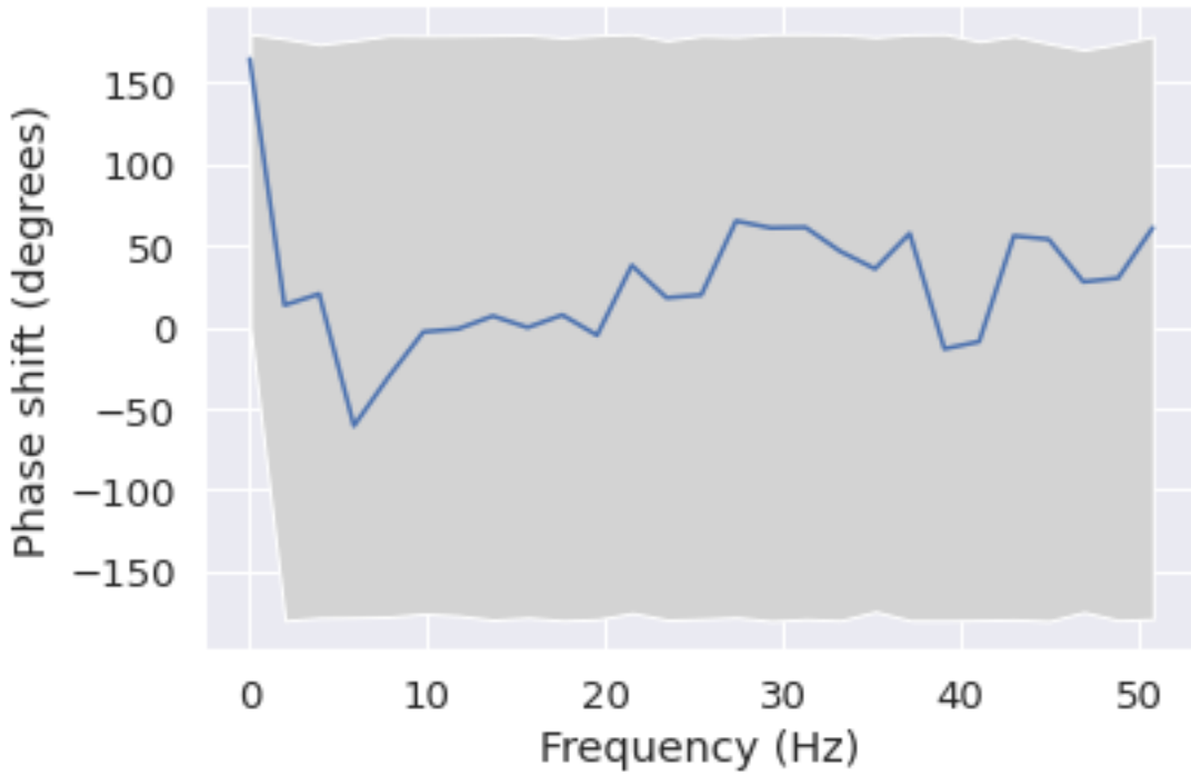
Phase shift for each frequency from Fz to O1
