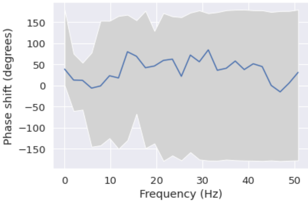
Phase shift for each frequency from T6 to T5
