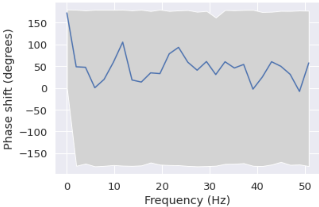
Phase shift for each frequency from P3 to Fp1
