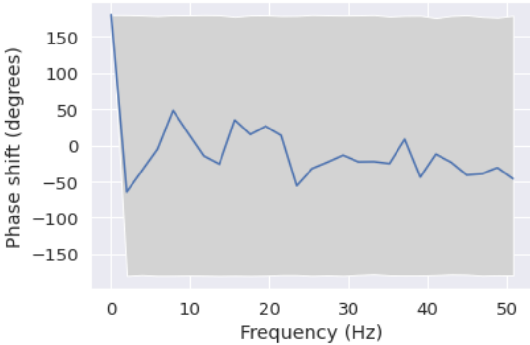
Phase shift for each frequency from F4 to P4
