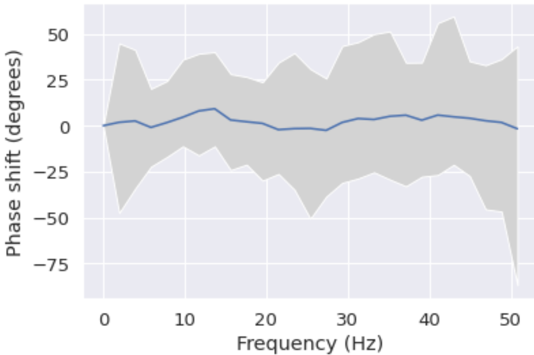
Phase shift for each frequency from F3 to Cz
