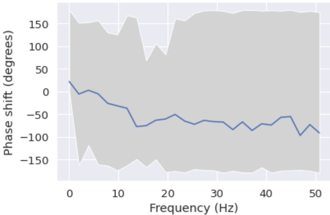
Phase shift for each frequency from T5 to Fz
