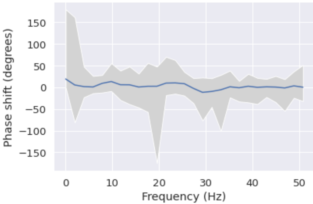
Phase shift for each frequency from C3 to F4
