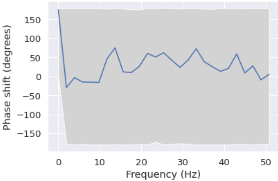
Phase shift for each frequency from T6 to C4
