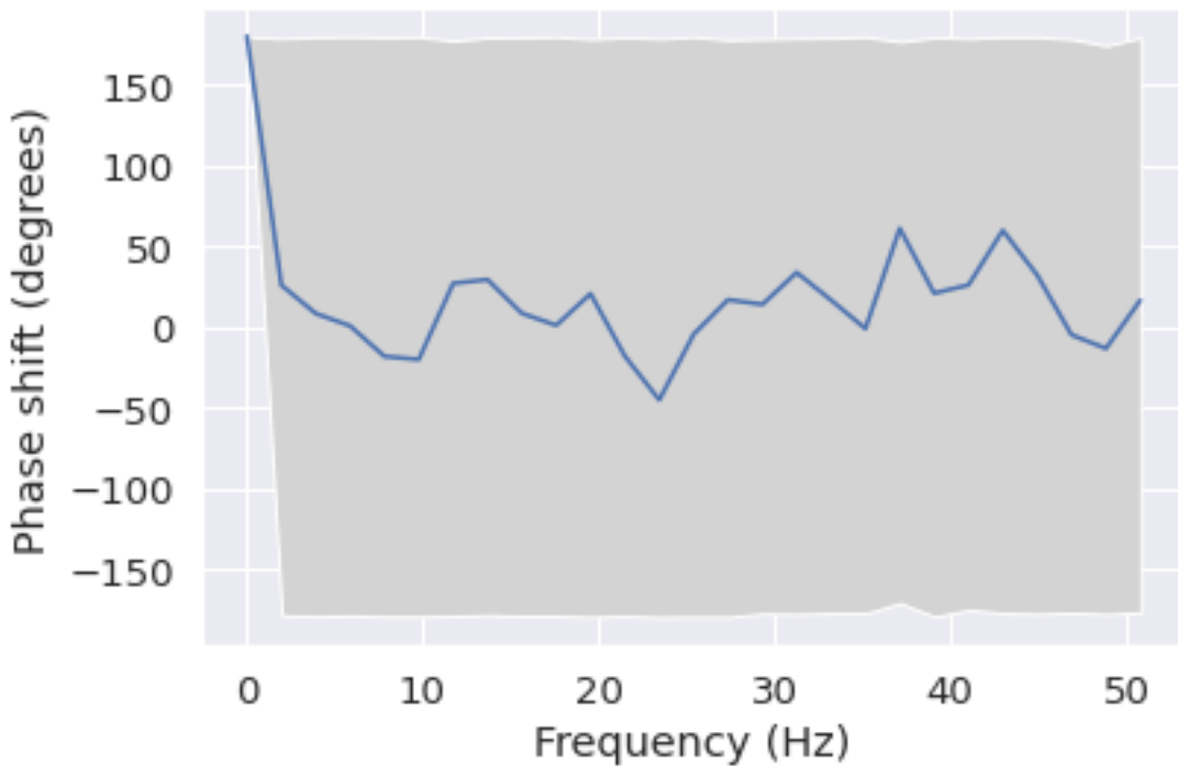
Phase shift for each frequency from P3 to F4
