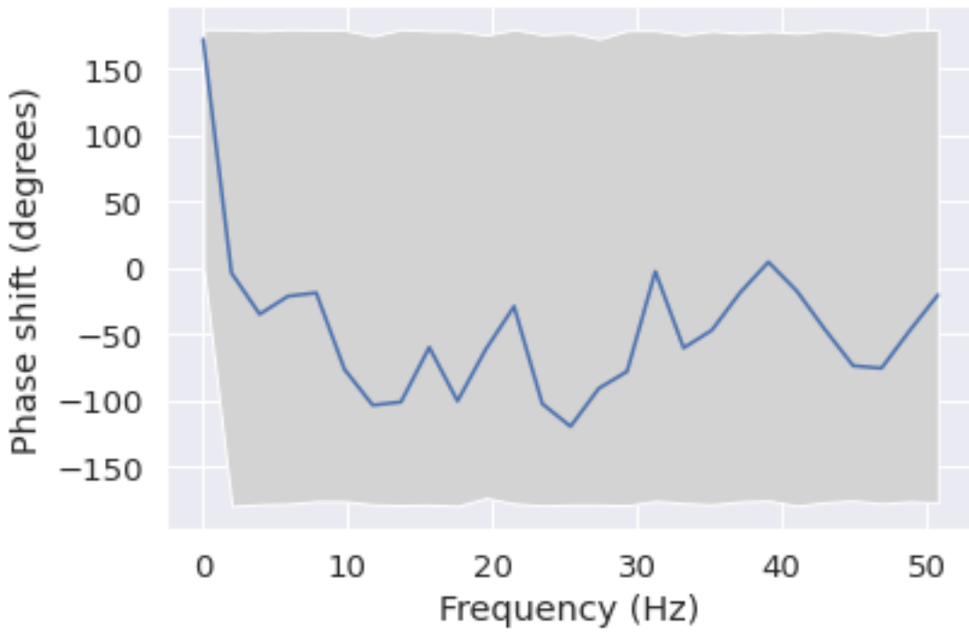
Phase shift for each frequency from T6 to Cz
