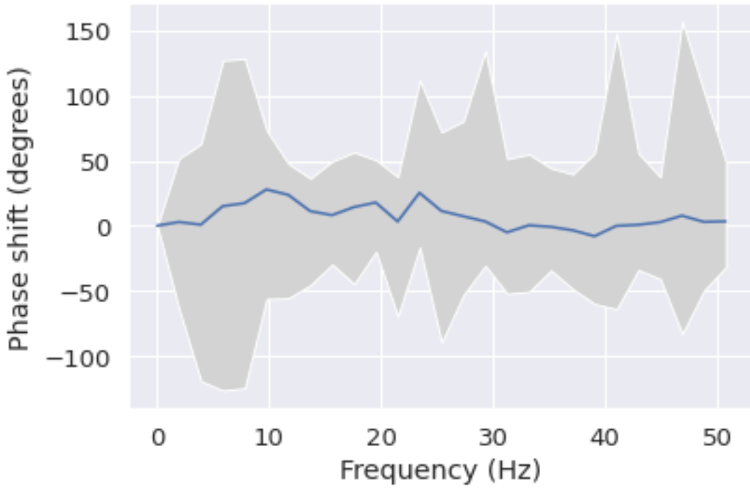
Phase shift for each frequency from P3 to C4
