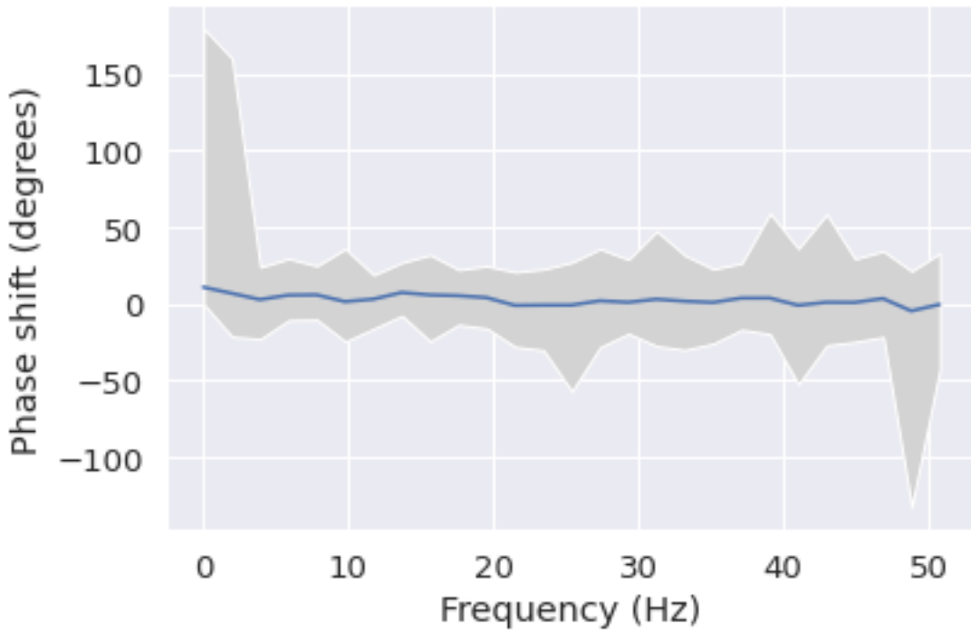
Phase shift for each frequency from F7 to Fp1
