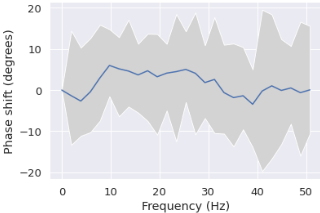
Phase shift for each frequency from O1 to T6
