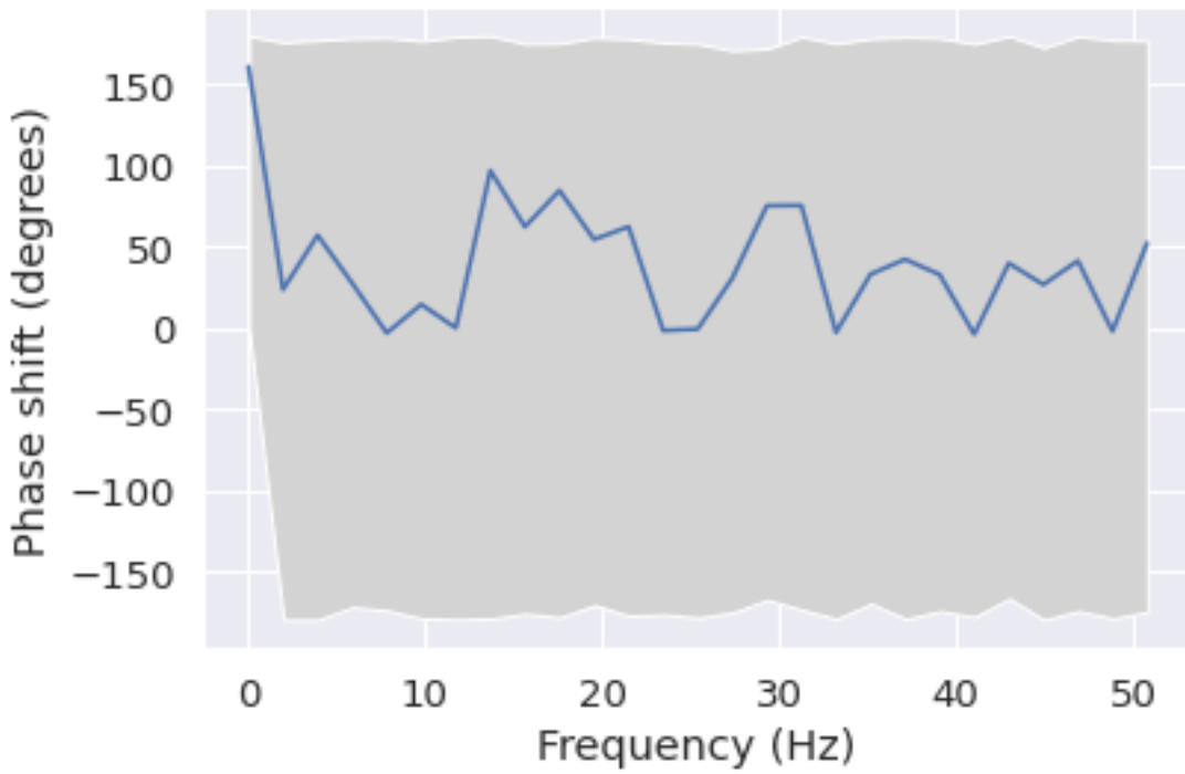
Phase shift for each frequency from F4 to Fz
