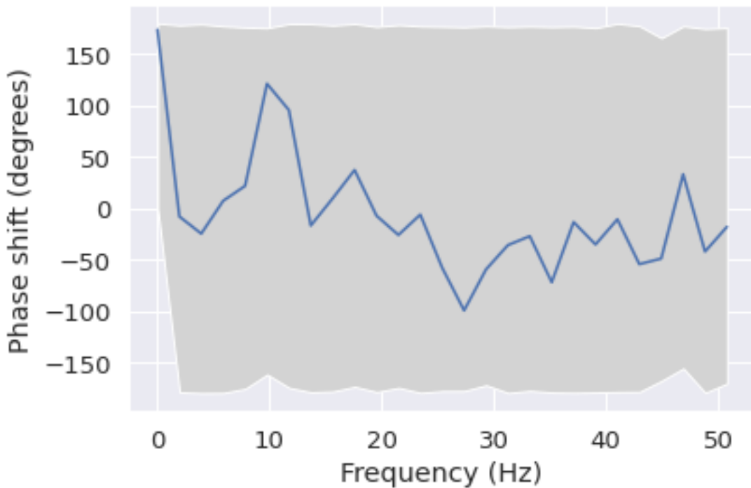
Phase shift for each frequency from C4 to Fp1
