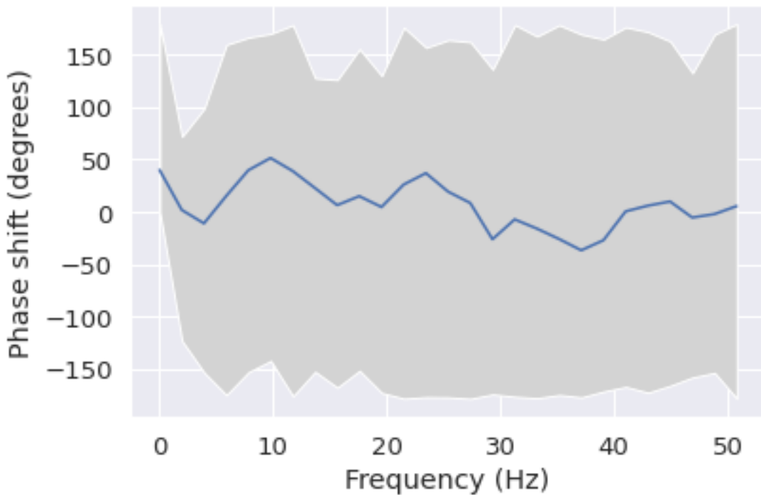
Phase shift for each frequency from Pz to C3
