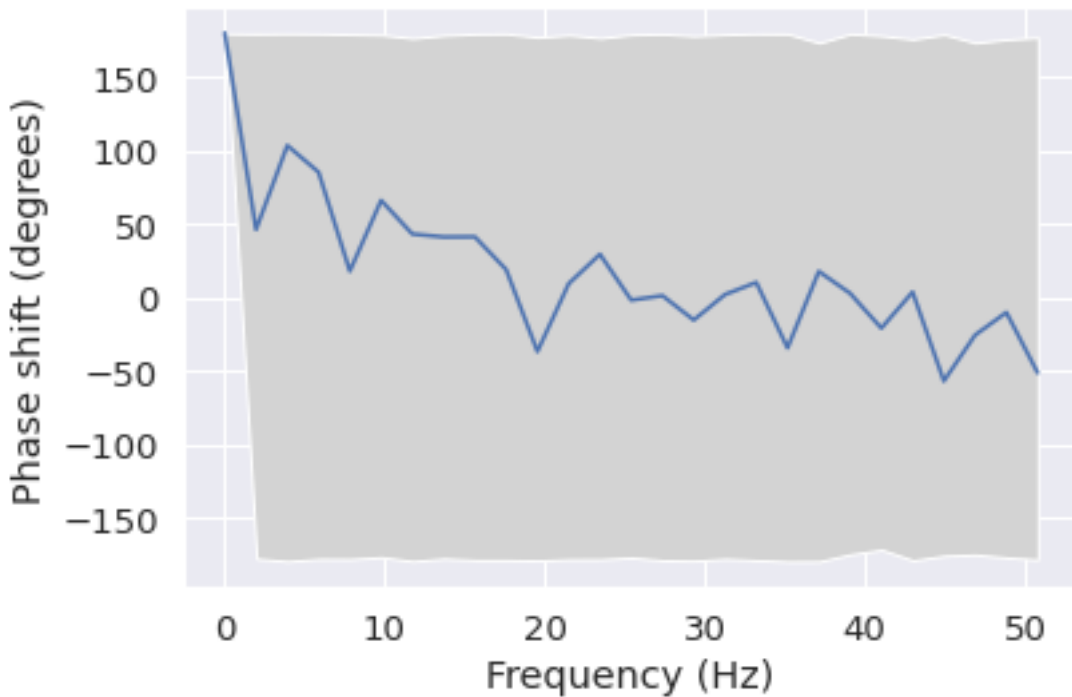
Phase shift for each frequency from C3 to T4
