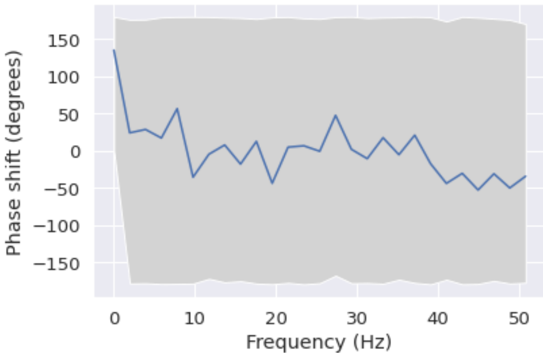
Phase shift for each frequency from C4 to C3
