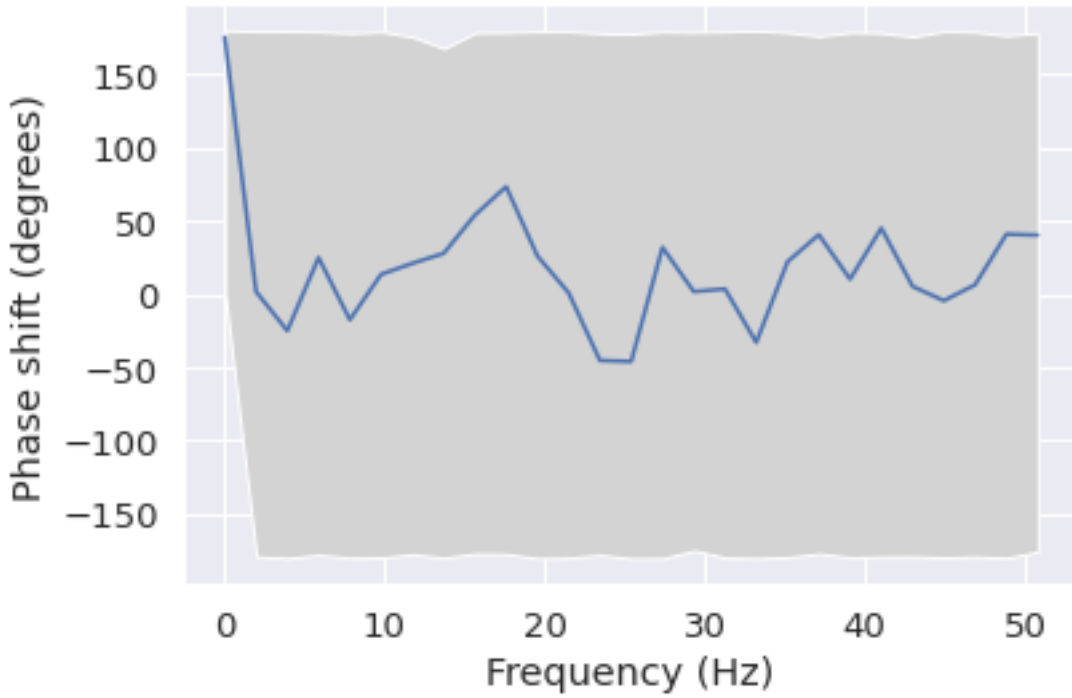
Phase shift for each frequency from O1 to F4
