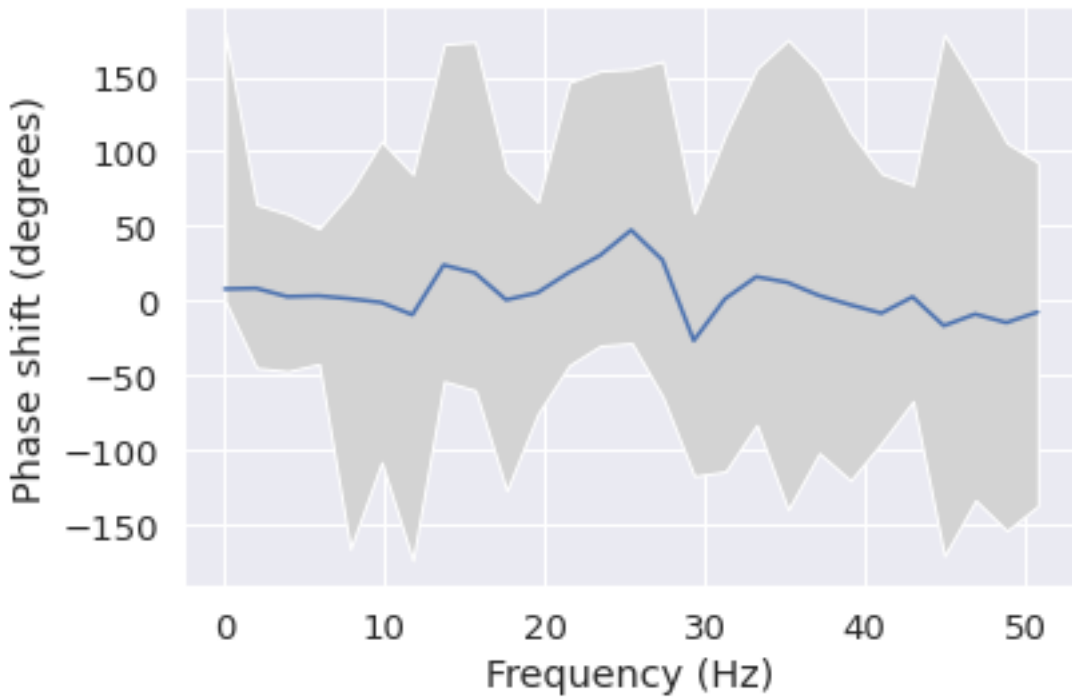
Phase shift for each frequency from C4 to Pz
