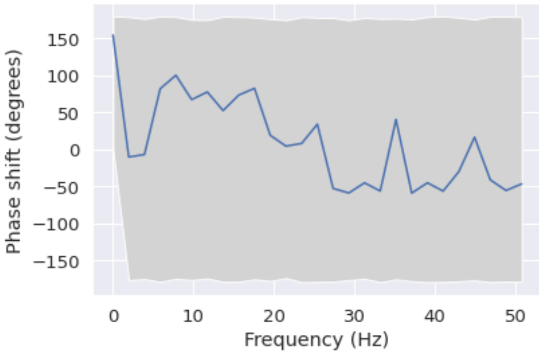
Phase shift for each frequency from F7 to Fz
