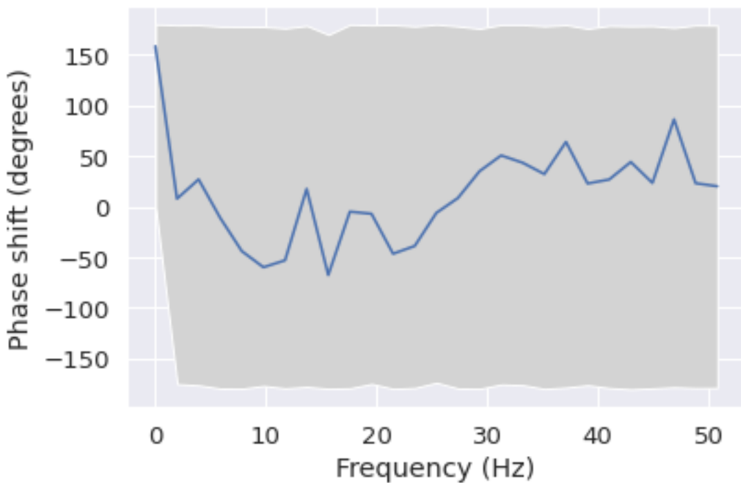
Phase shift for each frequency from T6 to F7
