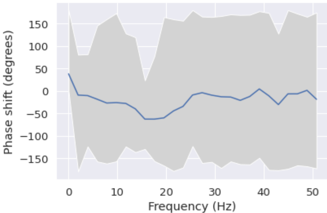
Phase shift for each frequency from F7 to T5
