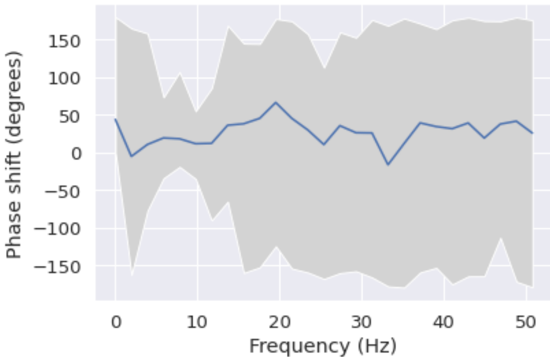
Phase shift for each frequency from T4 to P4
