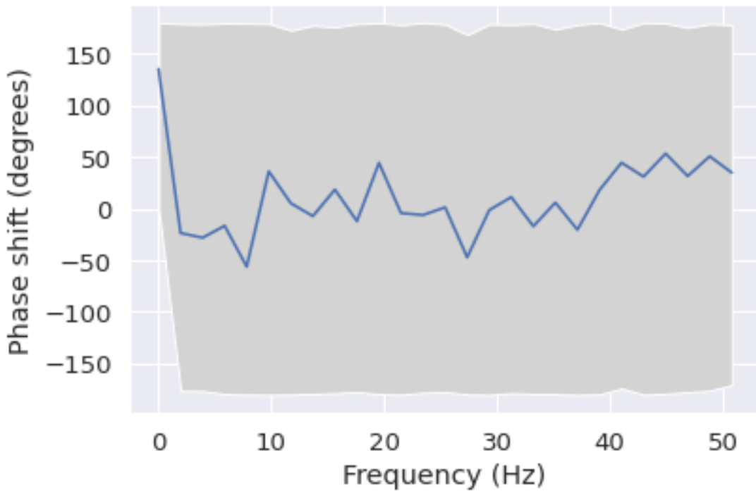
Phase shift for each frequency from C3 to P3
