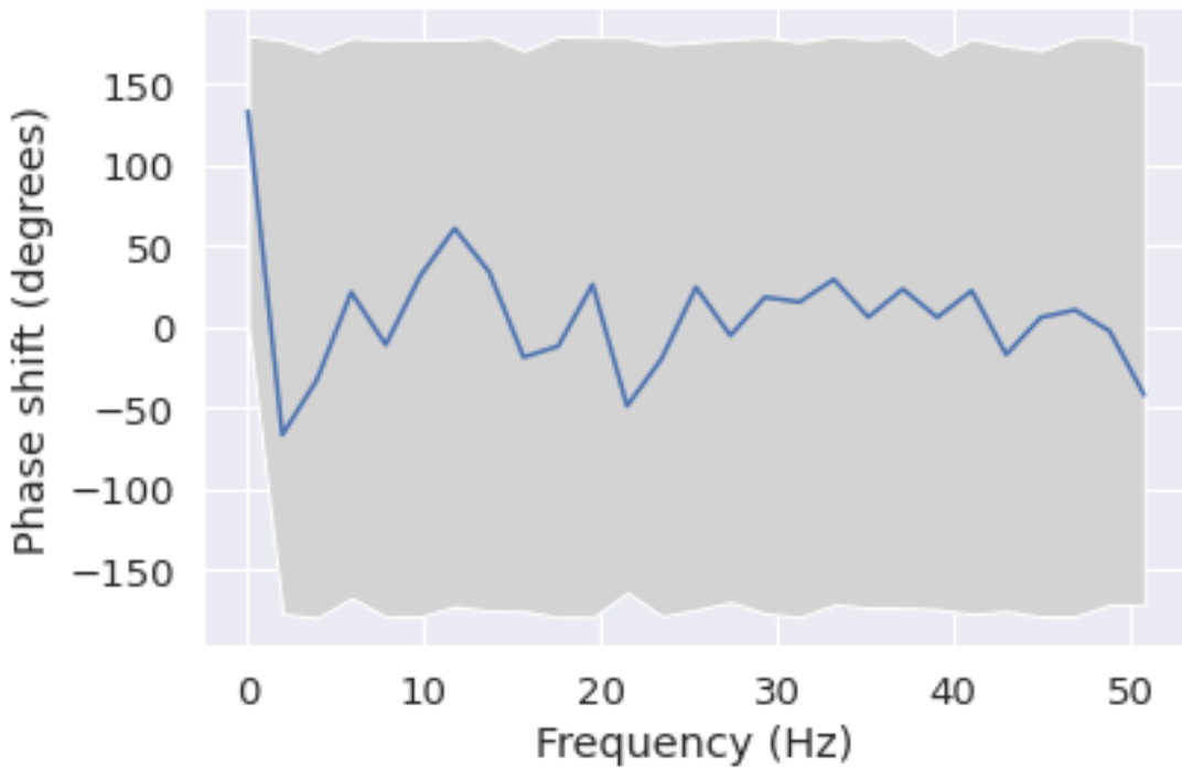
Phase shift for each frequency from Cz to T5
