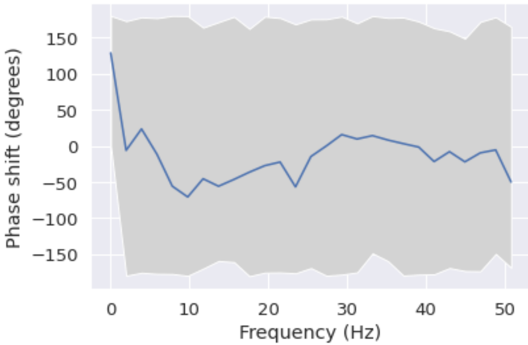
Phase shift for each frequency from T4 to Cz
