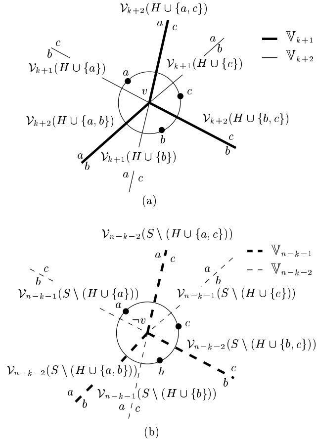
Figure 1: Incident edges: (a) v on the front range and (b) \neg v on the back range.
