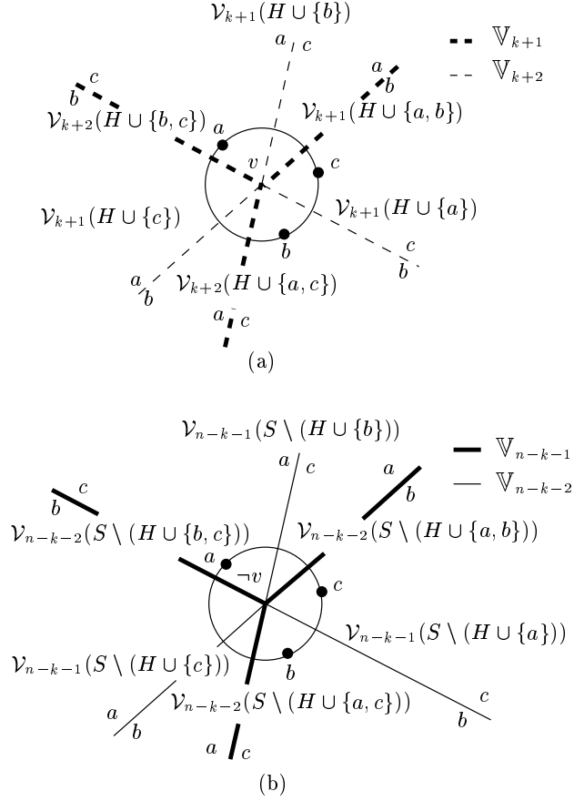
Figure 2: Incident edges: (a) v on the back range and (b) \neg v on the front range.
