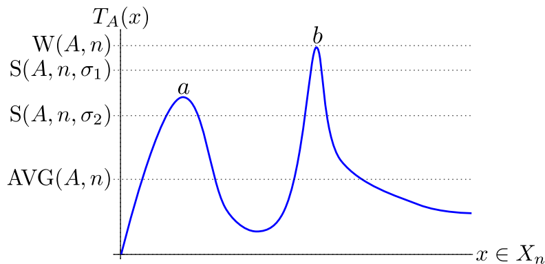
Figure 4.1: Illustration of different complexity analysis of the same algorithm A . The magnitude \sigma_1 is lower than \sigma_2 .
