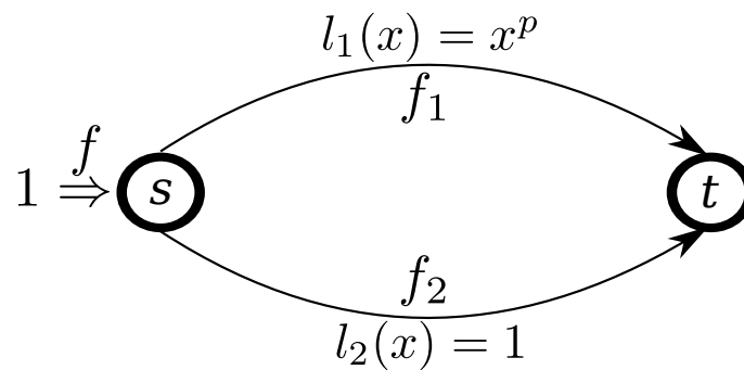
Figure 3.2: Pigou instance with polynomial latency functions.
