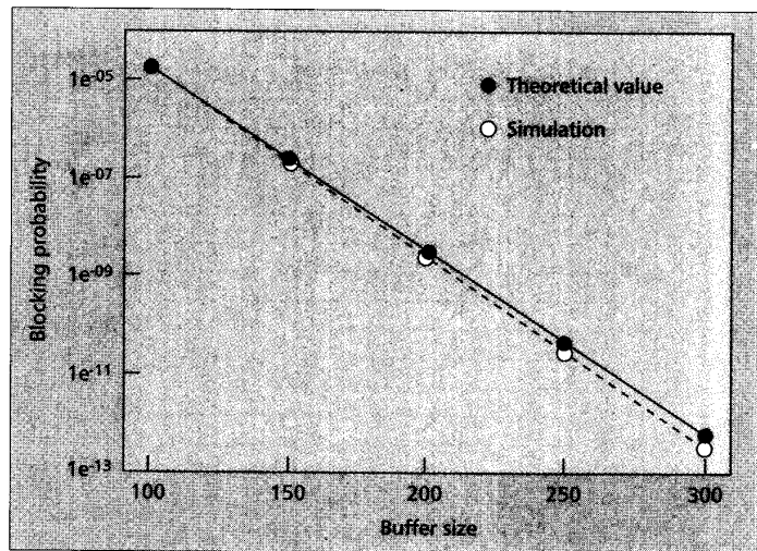
■ Figure 3. Importance sampling: blocking probability vs. buffer size. (Single server; eight biased sources with total load of 0.35 and burstiness of 8; eight unbiased sources with total load of 0.15 and burstiness of 4; run length: 5000 regenerative cycles; exponential bias with bias choice based on normalized sample variance.)
