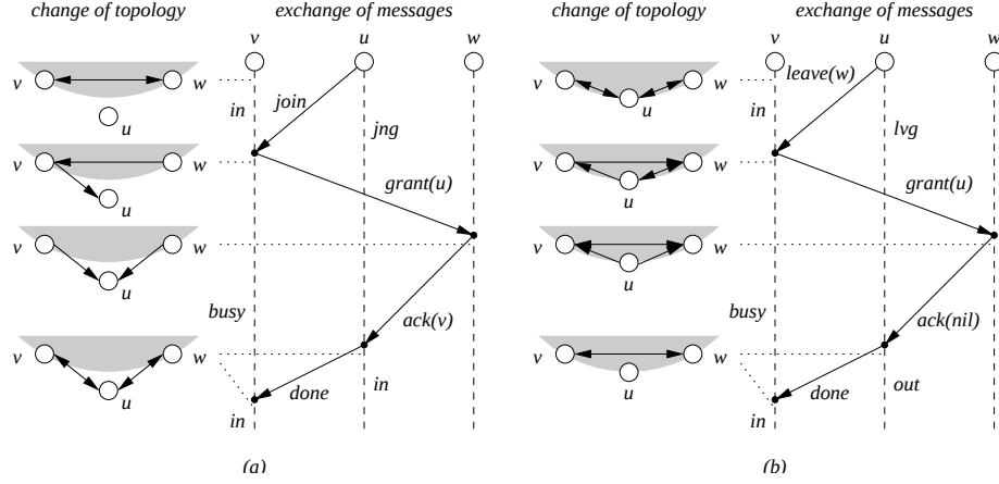
Fig. 3. Joining and leaving a bidirectional ring: (a) join, (b) leave.
