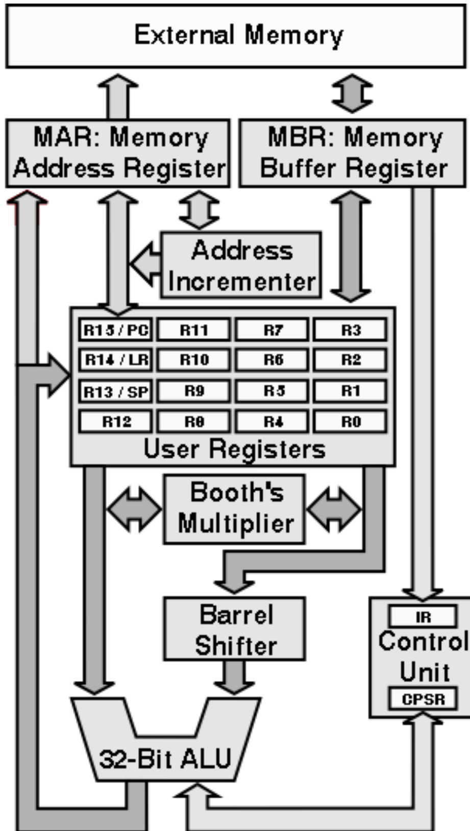
Figure 3.1: ARM Block Diagram
