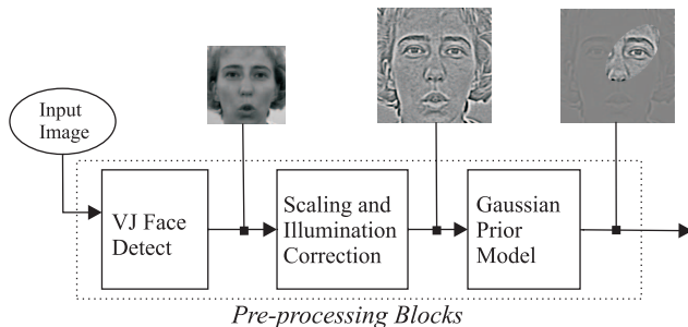
Fig. 2. The pre-processing steps.
