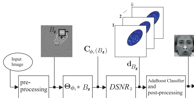
Fig. 3. The image, after pre-processing, will be processed through a sliding window B_{\mathbf{z}} , where \mathbf{z} is the coordinate corresponding to the center of the block. \mathbf{C}_{\phi_i}(B_{\mathbf{z}}) is obtained by filtering B_{\mathbf{z}} with each \Theta_{\phi_i} , where i = \{1, \dots, k\} , k being the number of principal components. The output of the box DSNR_2 provides the DSNR_2 (equation (1)) for each \mathbf{C}_{\phi_i}(B_{\mathbf{z}}) . So, each block B_{\mathbf{z}} has a DSNR_2 vector associated called \mathbf{d}_{B_{\mathbf{z}}} . The classifier generated with the AdaBoost algorithm will use \mathbf{d}_{B_{\mathbf{z}}} to classify B_{\mathbf{z}} . Finally, we perform a post-processing step consisting of scaling to original image size and a simple clustering algorithm to group the close labels.
