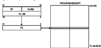
Figure 11. Direct Program Memory Addressing
