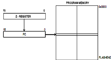
Figure 12. Indirect Program Memory Addressing
