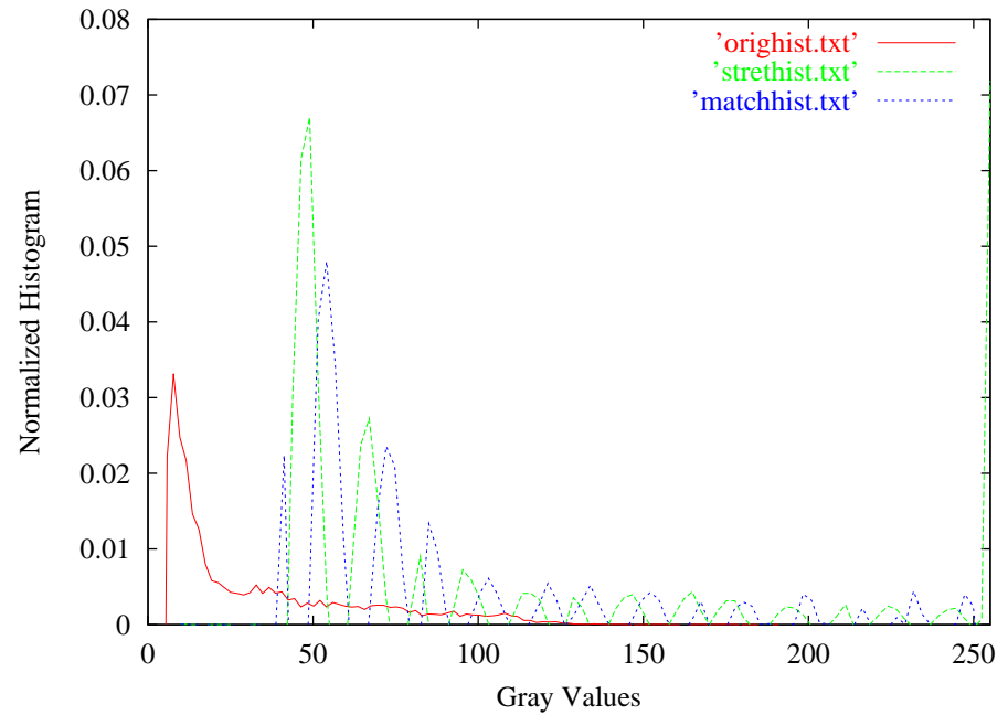
(b) Orig., stret. and matched histograms
